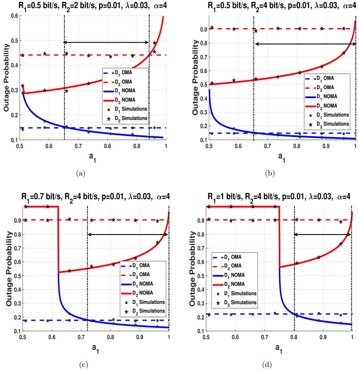
Figure 2.9.: Outage probability as a function of a_1 using cooperative NOMA and cooperative OMA for several value of data rates. (a) \mathcal{R}_1 = 0.5 bits/s and \mathcal{R}_2 = 2 bits/s. (b) \mathcal{R}_1 = 0.5 bits/s and \mathcal{R}_2 = 4 bits/s. (c) \mathcal{R}_1 = 0.7 bits/s and \mathcal{R}_2 = 4 bits/s. (d) \mathcal{R}_1 = 1 bits/s and \mathcal{R}_2 = 4 bits/s.
