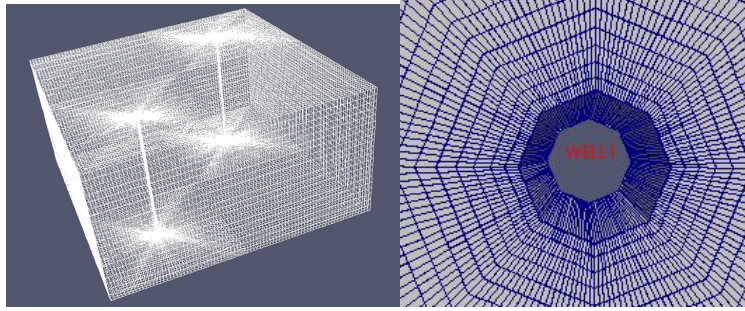
Figure 5.9: Mesh refinement near wells. The mesh is constructed in a manner to preserv conformity which is an important point for computational efficiency.
