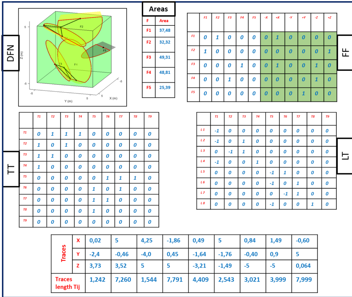
Figure 3.4: Output of the Connectivity Algorithm: the DFN containing five fractures, the adjacency matrix ( FF ), the trace-to-trace matrix ( TT ), the links-to-traces matrix ( LT ), the traces mid-points coordinates ( T ) and the traces vector ( T_{ij} )
