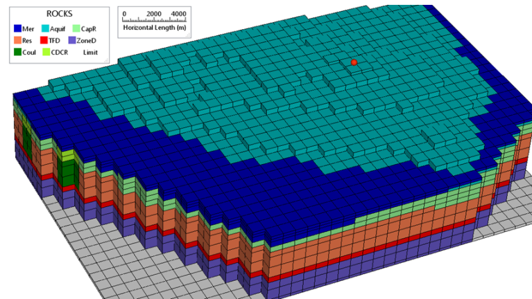
Figure 5.12: Conceptual model for the Vieux-Habitants Reservoir (GEOTREF project), adapted from [Garcia et al. (2018)].
