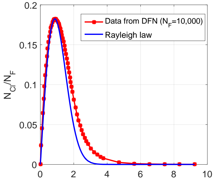
Figure 4.5: Rayleigh law for describing the cluster evolution in a DFN. The DFN contains 10,000 fractures.
