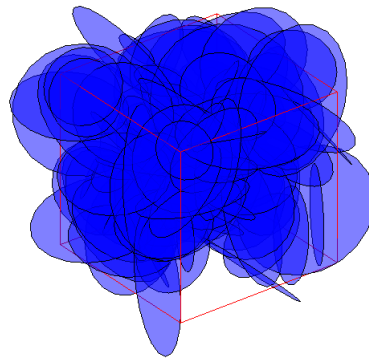
Figure 1.4: 3D Poissonian statistically isotropic fracture network with constant fracture size: this network has been generated with an in-house e matlab code for fracture network generation.
