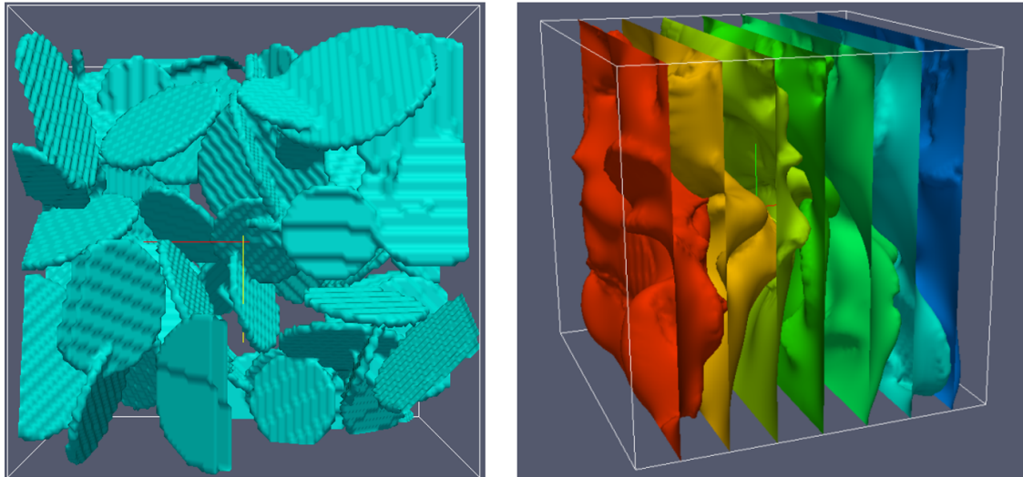
Fig. 3 Left: structured 3D Finite Volume Mesh (FVM) display of the fractured porous domain, with N = 125 planar disc fractures, and N_{\text{cells}} \approx N_1 \times N_2 \times N_3 \approx 106 cells. Right: numerical flow simulation using the Finite Volume BIGFLOW 3D code (iso-surfaces of hydraulic head are shown)
