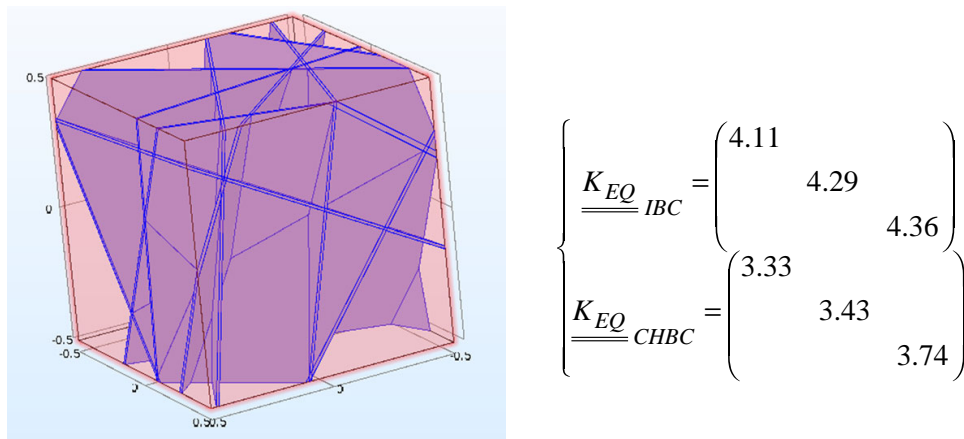
Fig. 5 Left: fracture network composed of “infinite” fractures (all fractures completely intersect the homogenization domain). Right: equivalent hydraulic conductivity tensor \underline{K}_{EQ} obtained for the two boundary conditions [immersion (IBC) and constant heads (CHBC)]
