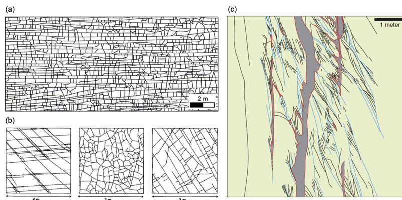
Figure 1.3: Geologically-mapped DFN patterns based on (a) a limestone outcrop at the south margin of the Bristol Channel Basin, UK, (b) sandstone exposures in the Doureay area, Scotland, and (c) fault zone structures in the Valley of Fire State Park of southern Nevada, USA. From [Lei et al. (2017)].
