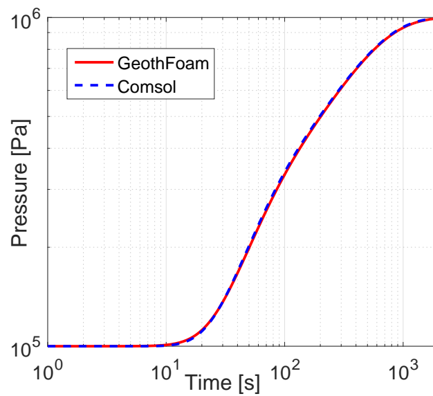
Figure 5.4: Pressure evolution comparison between GeothFoam and Comsol solvers. The boundary conditions are of Dirichlet type in x=0 and no-flow elsewhere. There is no source term in this case. The permeability of the medium is isotropic and homogeneous K = 1e^{-12}m^2 . The CPU times of the simulation is 9 and 10s for GeothFoam and Comsol respectively.
