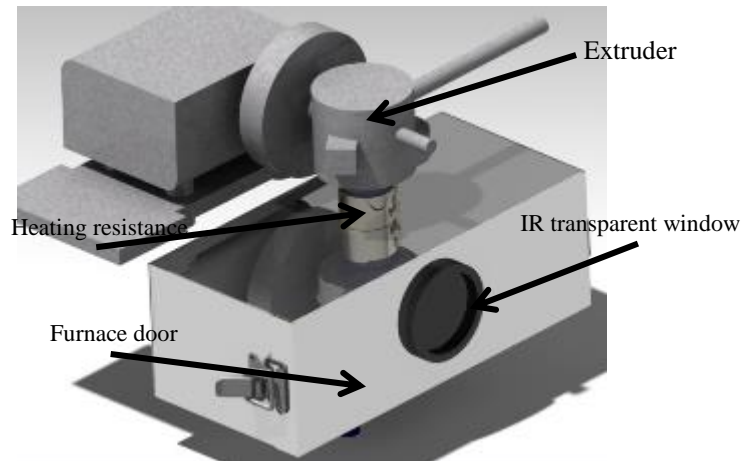
Figure 17: Heating furnace designed according to the design criteria
