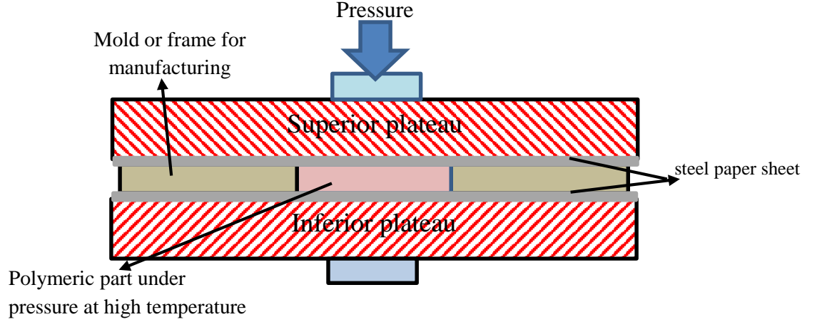
Figure 20: Schematic illustration of the hot compression press used to manufacture the polymeric plates
