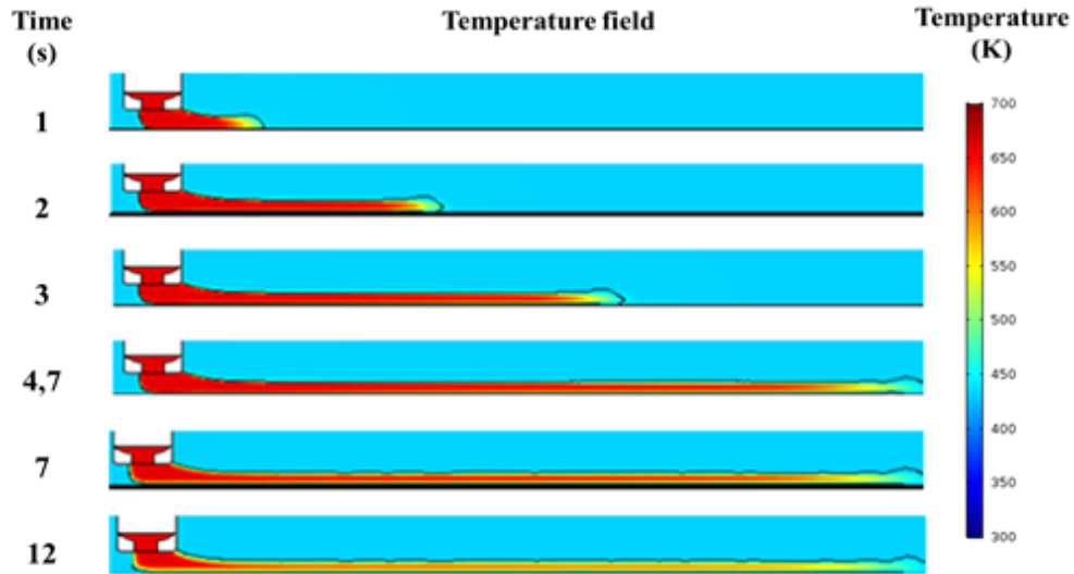
Figure 88: Temperature distribution for the Case 3 ( T_{\text{substrate}} = 433\text{K} and T_{\text{env.}} = 433\text{K} )
