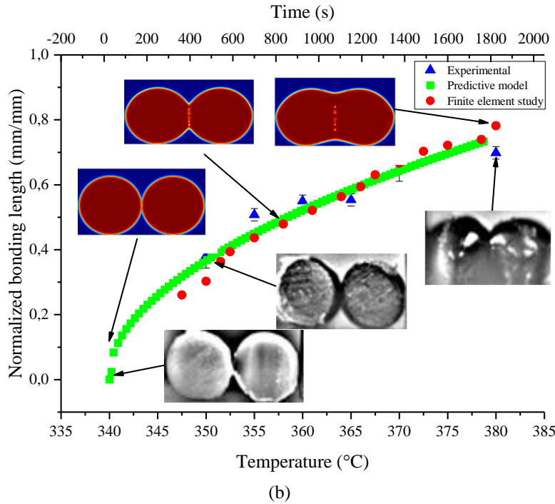
Figure 39: Evolution of the coalescence of the filaments according to temperature for PEEK
