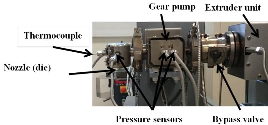
Figure 7: Extruder system
