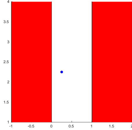
Figure 5.2.2: 2D parallel zero flux interfaces
