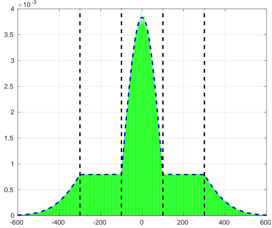
Figure 3.4.4: Comparison between analytical (PDE) and numerical (RWPT) concentration histogram using negative particles, for a 1D infinite domain with an initial Dirac mass at x_0 = 0 (“source”). The diffusion and the porosity coefficients D(x) and \theta(x) are discontinuous at the black dashed lines (see Table 3.2). The dashed blue curve is the semi-analytical solution of the diffusion (See subsection 3.3.6.1). The histogram is the result obtained by the RWPT with ten million initial particles. The diffusion and porosity contrasts are given in Table 3.2. This result was obtained by setting the time step equal to the final simulation time, for more efficiency and minimum calculation time.
