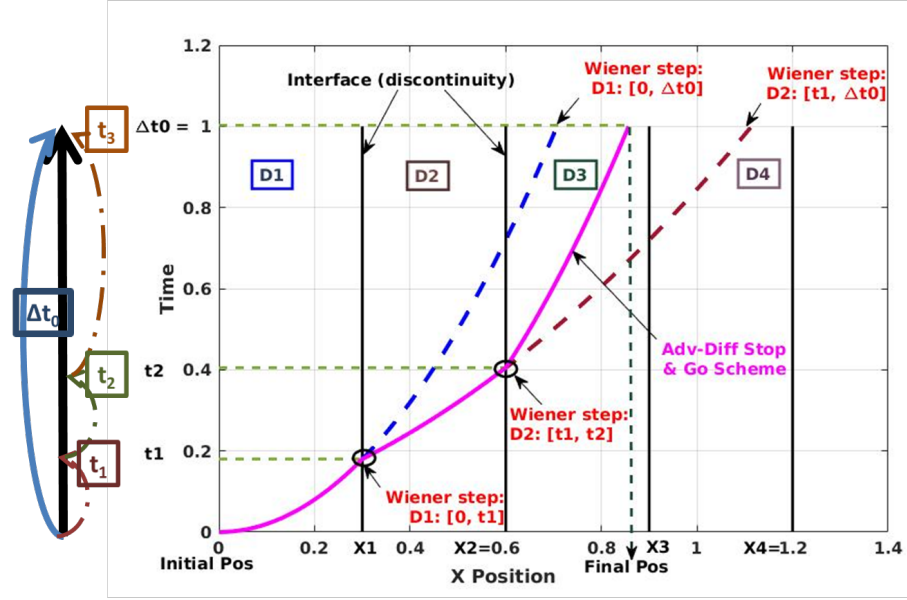
Figure 3.3.3: Time step splitting scheme: Left (vertically): macro-time step \Delta t_0 , and intermediate steps t_1, t_2, t_3 . Right: schematic space-time graph illustration of the position of a particle, in one macro-time step \Delta t_0 , that crosses many interfaces in a domain with different diffusion coefficients.
