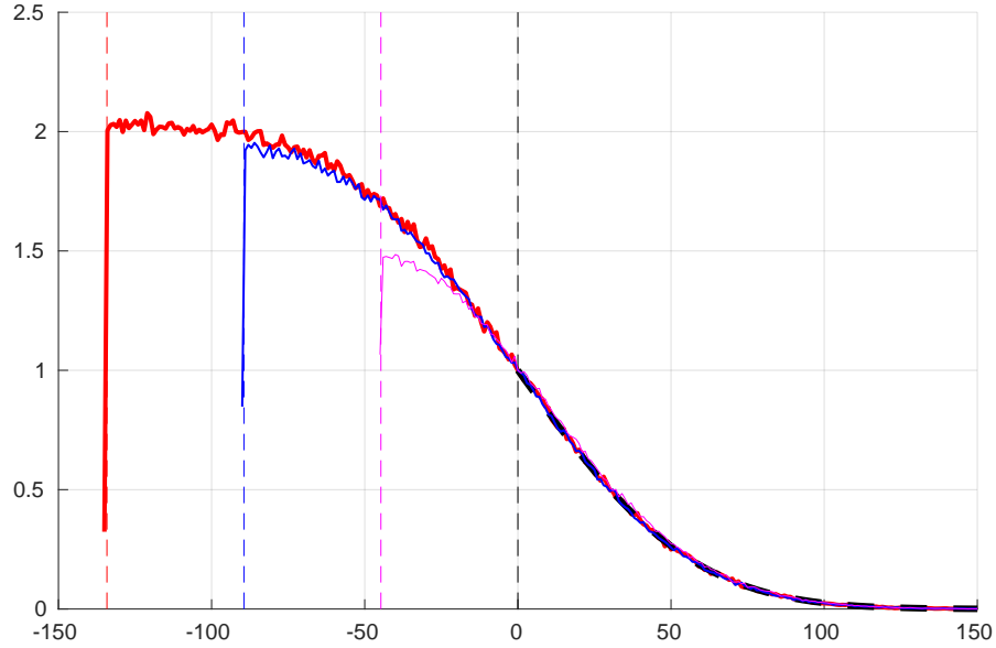
Figure 4.4.5: Concentration profiles using the External Semi-Reservoir method: The red, blue and magenta curves represent the concentrations with a Semi-Reservoir with a size of 3\sqrt{2Dt} , 2\sqrt{2Dt} , \sqrt{2Dt} respectively. The black dashed curve represents the analytical solution for a semi-infinite domain with a Dirichlet BC.
