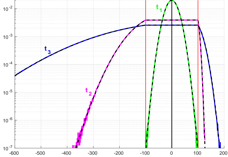
Figure 3.4.8: Time evolution of concentration profiles using the Stop & Go algorithm. The red bold lines correspond to the position of the interfaces x = -100 and x = 100 . The green, magenta and blue bold curves correspond to the result of the simulation of the negative unit mass method at three different times t_1 , t_2 , t_3 respectively. The dashed black curves correspond to the corresponding semi-analytical solutions described in subsection 3.3.6.1.
