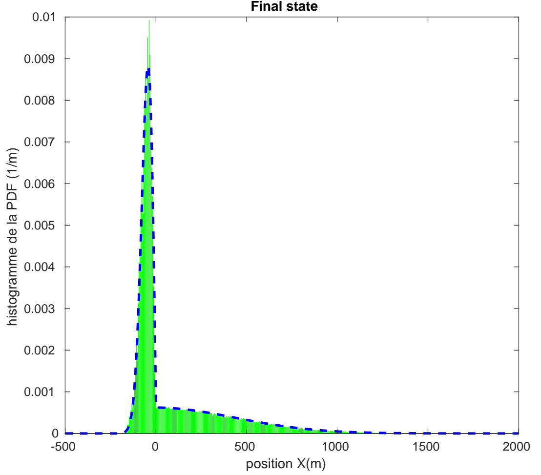
Figure 3.4.1: Comparison between analytical (PDE) and numerical (RWPT) concentration histogram using Reflection/Refraction particles, for a 1D infinite domain with an initial Dirac mass at x_0 = -1 (“source”). The diffusion coefficient D(x) and porosity \theta(x) are discontinuous. The dashed blue bold curve is the analytical solution of the diffusion PDE, Eq.3.2.19. The slightly fluctuating histogram is the result obtained by the RWPT with 100,000 particles. The diffusion contrast is D_2/D_1 = 100 and the porosity contrast \theta_2/\theta_1 = 100 .
