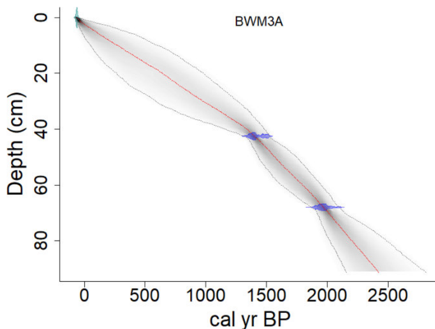
Figure 46: Age-depth model of BWM core. Red dotted line=median age, grey shaded area=95% confidence interval.
