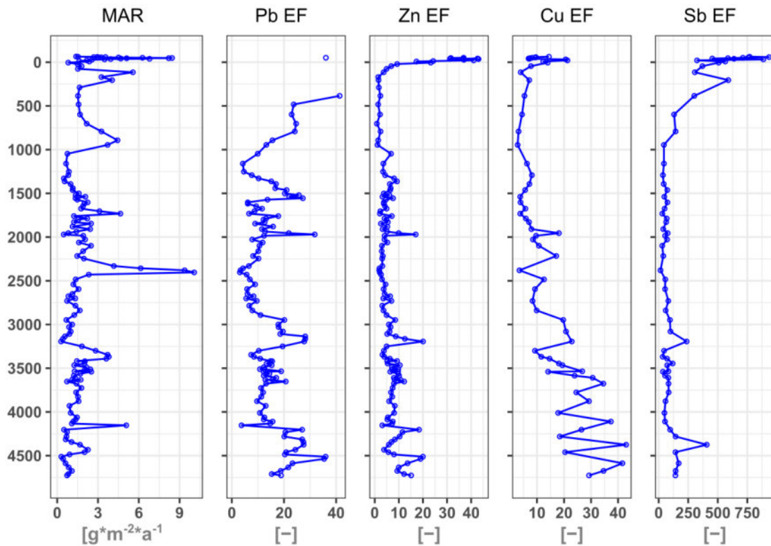
Figure 34: Chronological profiles of MAR, EF Pb (clipped at 10 % of max. EF), EF Zn, EF Cu and EF Sb in Pi17.
