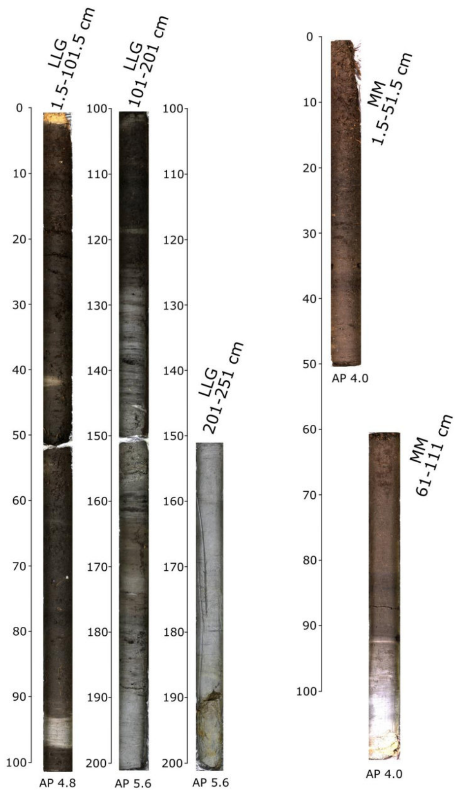
Suppl. Figure 3: Line-scans of Fimba Valley core-sequences (LLG, MM). AP= line-scan camera aperture.
