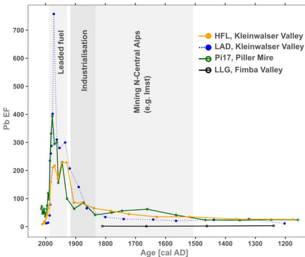
Figure 58: Pb EF since the Late Middle Ages of HFL, LAD, LLG and Pi17.
