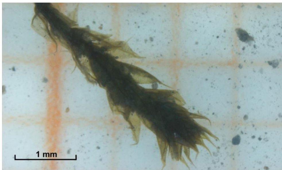
Figure 43: Brown moss from LLG, depth of 162-163 cm, selected for dating (Poz-91984), with grey mineral particles.
