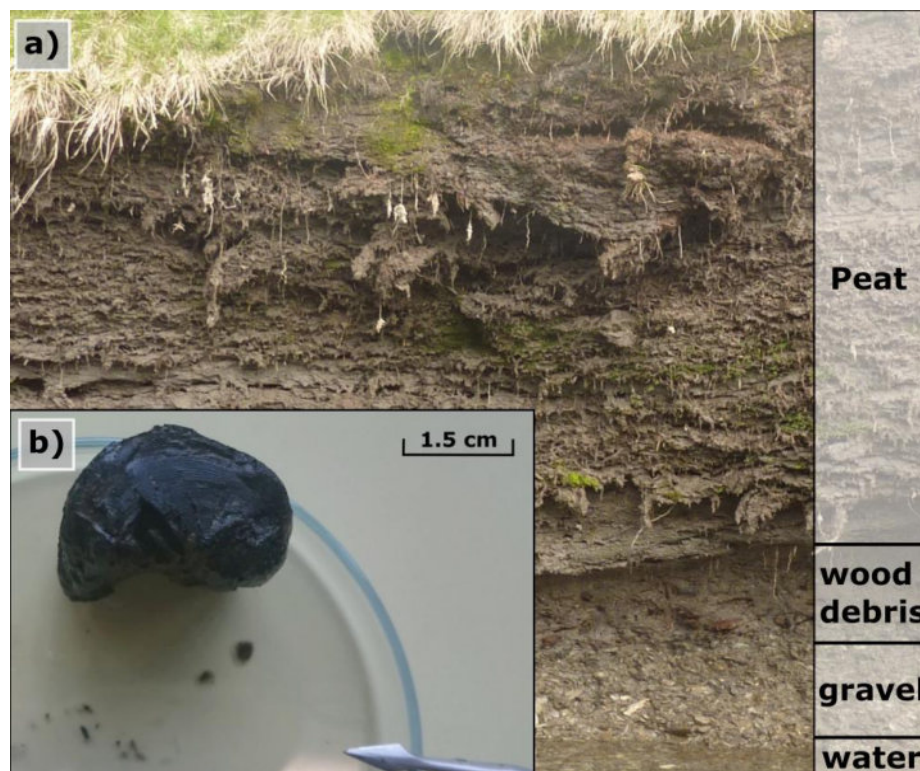
Figure 9: Open profile of HHA and charred wood radiocarbon sample. Tree rings counted to approx. 60 years.
