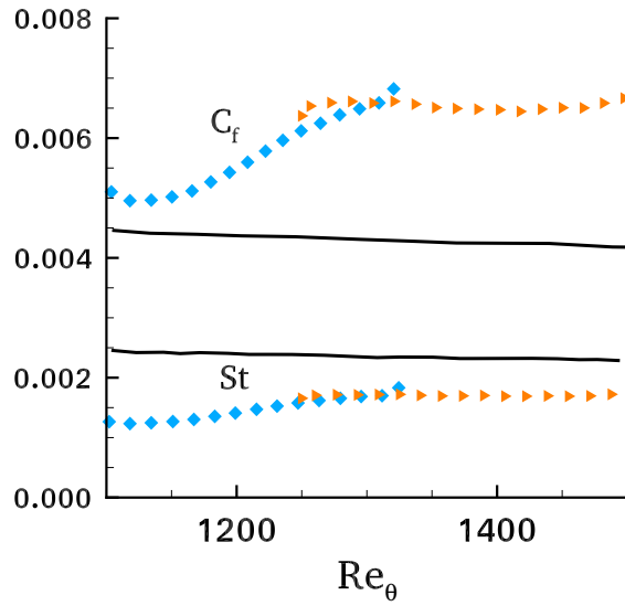
Figure 4.6: Streamwise variation of the skin friction coefficient C_f and the Stanton number St with Re_\theta , using Code-1 and Code-2. The influence of the extension in the streamwise direction. (solid lines) - Li et al. [58]; (◆) - Code-1, (▶) - Code-2.
