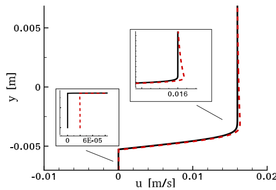
Figure 2.19: Evolution of the tangential velocity u for the vaporization study case for Pr = 1.022 , Re_{x_L} = 85.726 , \rho_l/\rho_v = 17.746 , Ja_{vap} = 3.69 : black line - Blasius theory, red dashed line - vaporization configuration. Zoom on the liquid region (the bottom left) and on the zone close to the interface (middle right).
