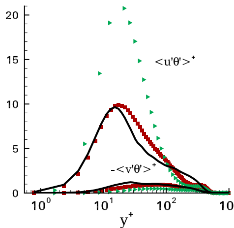
Figure 3.29: Turbulent heat fluxes in the streamwise \langle u'\theta' \rangle^+ and wall-normal \langle -v'\theta' \rangle^+ directions. Each curve is plotted after the corresponding T_{cv} . (black line) - the statistics of the imposed inlet inflow; ( \blacktriangleright ) - 256 \times 64 \times 64 ; ( \blacksquare ) - 512 \times 128 \times 128 .
