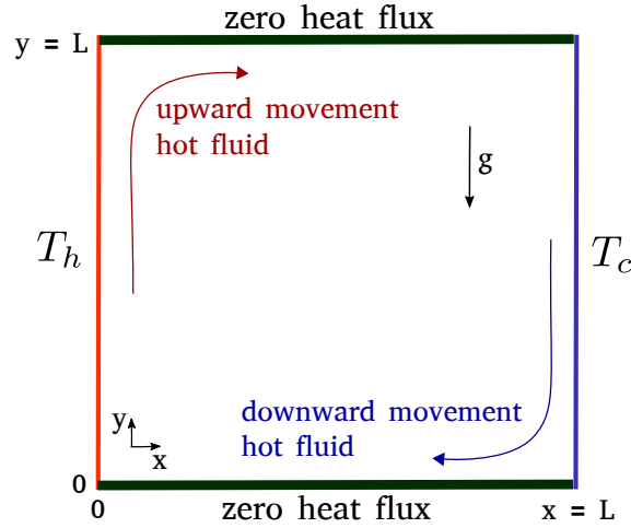
Figure 5.1: Differentially heated square cavity problem.
