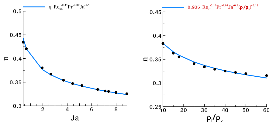
(c) Evolution with the Jakob number and keeping fixed the dimensionless numbers: Pr = 1.022 , Re_{x_L} = 85.7226 and \frac{\rho_l}{\rho_v} = 17.746 . // q(\frac{\rho_l}{\rho_v}) = 0.6567 . (d) Evolution with the density ratio and keeping fixed the dimensionless numbers: Pr = 1.022 , Re_{x_L} = 85.7226 and Ja = 3.69 .
