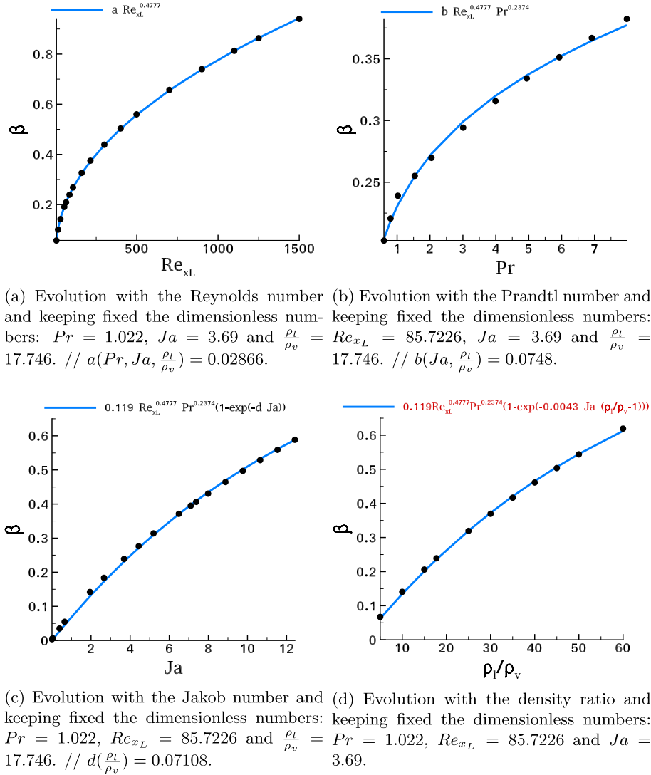
Figure C.18. Evolution of the jump \beta(Re_{x_L}, Pr, Ja, \frac{\rho_l}{\rho_v}) for x = x_L - Vaporization configuration.
