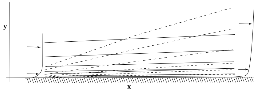
Figure 3.9: Sketch of the Spalart's approach to simulate a spatially developing boundary layer using periodic boundary conditions. The graph is extracted from Spalart [95]. (solid lines) - streamlines; (dashed lines) - coordinate lines.
