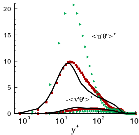
Figure 3.29: Turbulent heat fluxes in the streamwise \langle u'\theta' \rangle^+ and wall-normal \langle v'\theta' \rangle^+ directions. Each curve is plotted after the corresponding T_{cv} . (black line) - the statistics of the imposed inlet inflow; ( \blacktriangleright ) - 256 \times 64 \times 64 ; ( \blacksquare ) - 512 \times 128 \times 128 .
