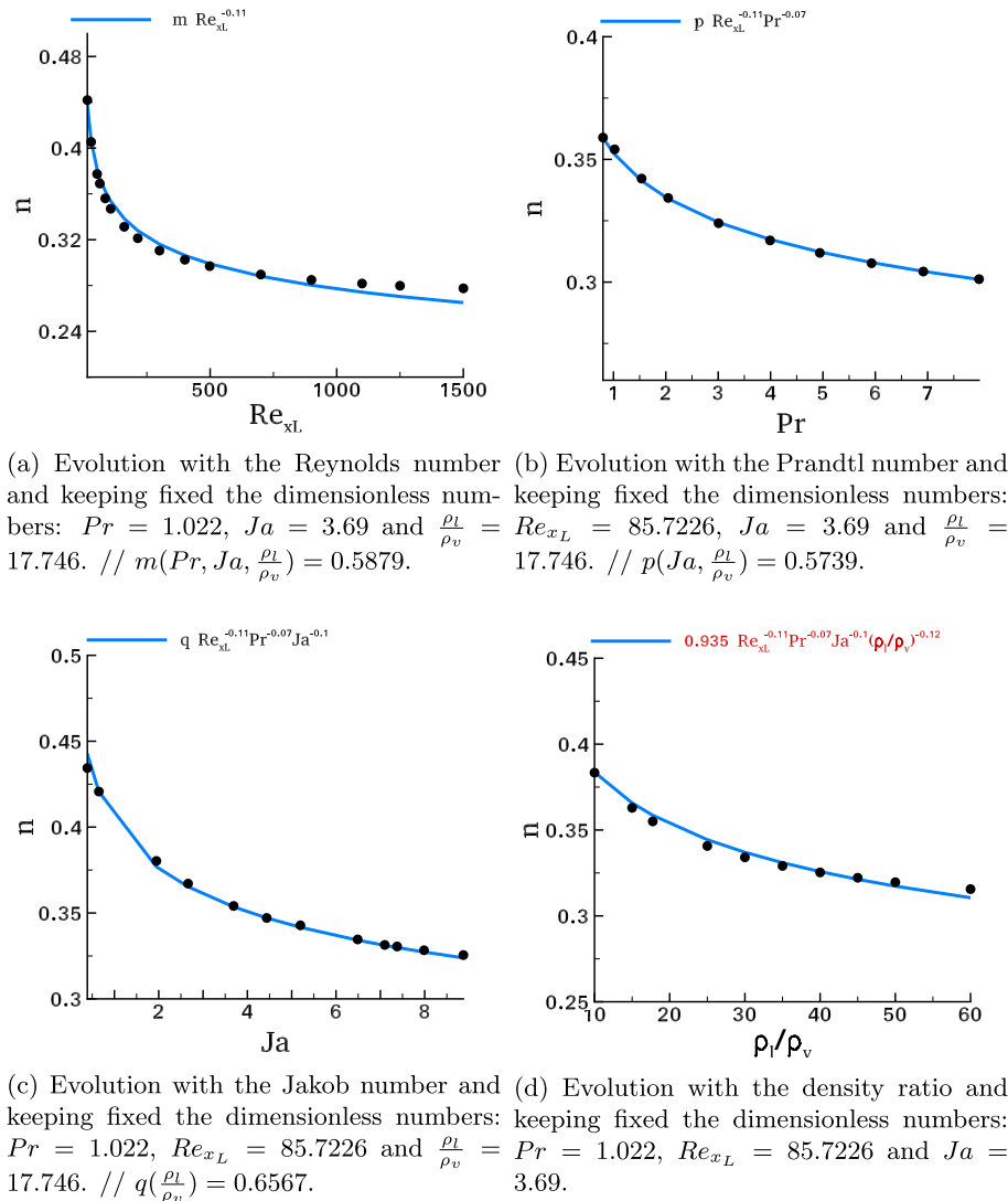
Figure C.21. Evolution of the parameter n(Re_{x_L}, Pr, Ja, \frac{\rho_L}{\rho_v}) for x > x_L - Vaporization configuration.
