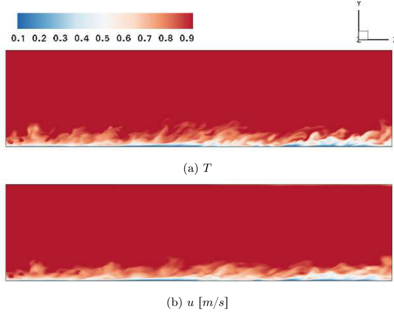
Figure 3.24: Reduced temperature and streamwise velocity fields for a spatially developing boundary layer over a flat plate. The caption is taken after 1528\theta_{inlt}/U_\infty = 480 s.
