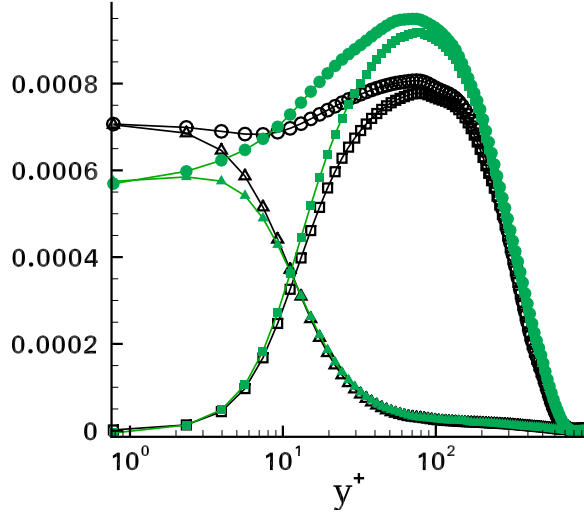
Figure 4.13: Shear stress distribution with the wall coordinate. The dimensionless numbers are Re_\theta = 1100 , Pr = 1.022 , \rho_l/\rho_v = 17.746 and two values of the Jakob number: (black colour) - Ja = 0 ; (green colour) - Ja = 0.88 ; (circle) - total shear stress; (square) - Reynolds shear stress; (triangle) - viscous shear stress.
