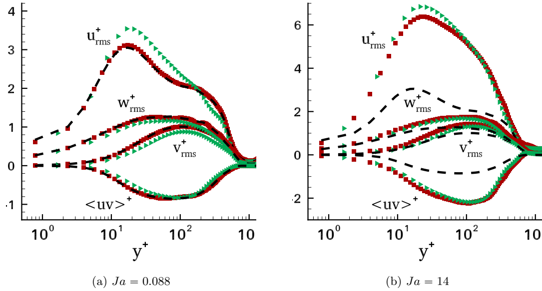
Figure C.2: Influence of the mesh grid onto the evolution of the rms quantities. ( \blacktriangleright ) - 256 \times 64 \times 64 ; ( \blacksquare ) 512 \times 128 \times 128 ; (dashed line) - without phase change with the mesh 512 \times 128 \times 128 .
