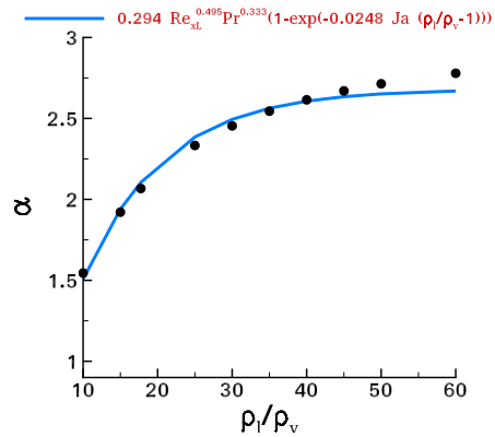
(c) Evolution with the Jakob number and keeping fixed the dimensionless numbers: Pr = 1.022 , Re_{x_L} = 85.7226 and \frac{\rho_L}{\rho_v} = 17.746 . // d(\frac{\rho_L}{\rho_v}) = 0.4185 . (d) Evolution with the density ratio and keeping fixed the dimensionless numbers: Pr = 1.022 , Re_{x_L} = 85.7226 and Ja = 3.69 .
