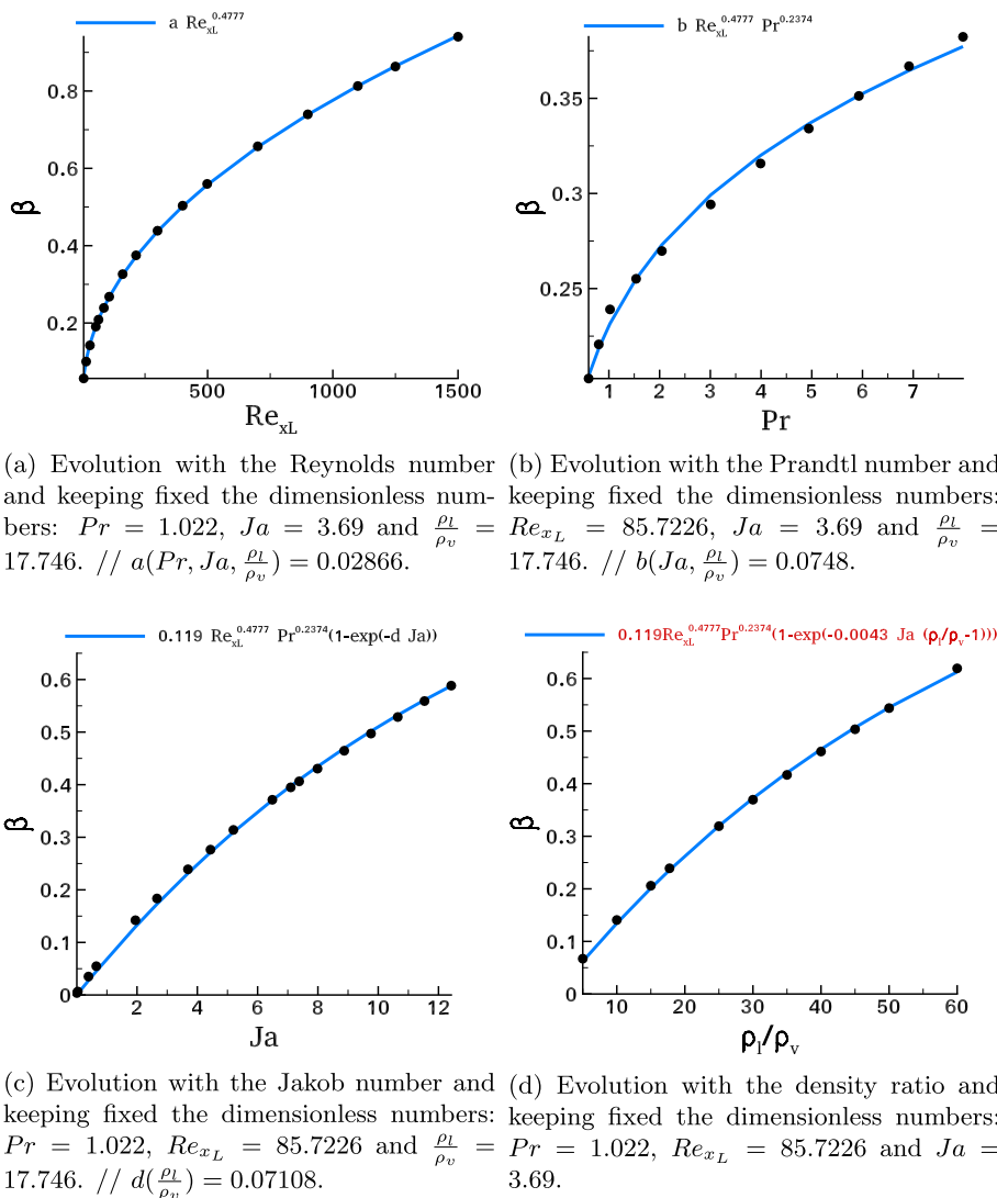
Figure C.18. Evolution of the jump \beta(Re_{x_L}, Pr, Ja, \frac{\rho_l}{\rho_v}) for x = x_L - Vaporization configuration.
