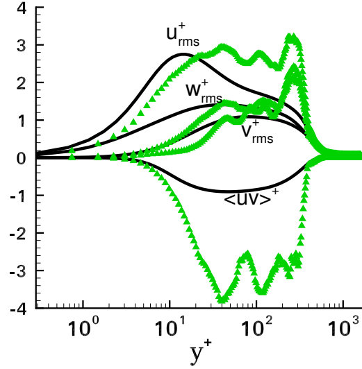
Figure B.4: Inlet plane statistics evolution with the wall coordinate obtained using the modified SEM, proposed by Pamies et al. [72]. (black line) - Jimenez data [40]; ( \blacktriangle ) - the obtained profiles.
