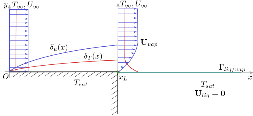
Figure 2.1: Schematics of the expanding Blasius-Pohlhausen boundary layer interacting with a saturated and static liquid pool.
