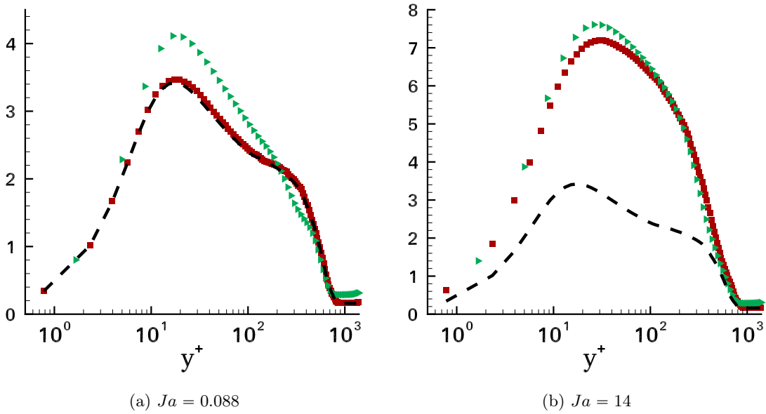
Figure C.3: Influence of the mesh grid onto the evolution of the rms temperature. ( \blacktriangleright ) - 256 \times 64 \times 64 ; ( \blacksquare ) 512 \times 128 \times 128 ; (dashed line) - without phase change with the mesh 512 \times 128 \times 128 .
