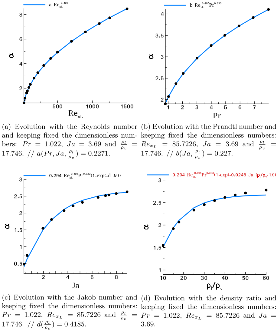
Figure C.20. Evolution of the coefficient \alpha(Re_{x_L}, Pr, Ja, \frac{\rho_L}{\rho_v}) for x > x_L - Vaporization configuration.
