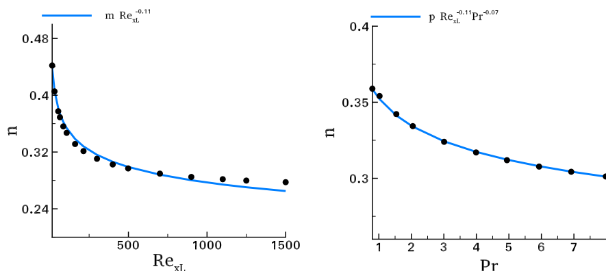
(a) Evolution with the Reynolds number and keeping fixed the dimensionless numbers: Pr = 1.022 , Ja = 3.69 and \frac{\rho_l}{\rho_v} = Re_{x_L} = 85.7226 , Ja = 3.69 and \frac{\rho_l}{\rho_v} = 17.746 . // m(Pr, Ja, \frac{\rho_l}{\rho_v}) = 0.5879 . (b) Evolution with the Prandtl number and keeping fixed the dimensionless numbers: Pr = 1.022 , Re_{x_L} = 85.7226 and \frac{\rho_l}{\rho_v} = 17.746 . // p(Ja, \frac{\rho_l}{\rho_v}) = 0.5739 .
