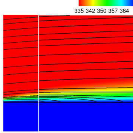
Figure 2.3: Streamlines and temperature profile [K] of a subcooled gas flow condensating in the liquid pool. for Pr = 0.98 , Re_{x_L} = 211 , \rho_l/\rho_v = 1623 , Ja_{cond} = 0.74 ; left - classic Blasius boundary layer, right - the boundary layer "aspirated" by the condensation.
