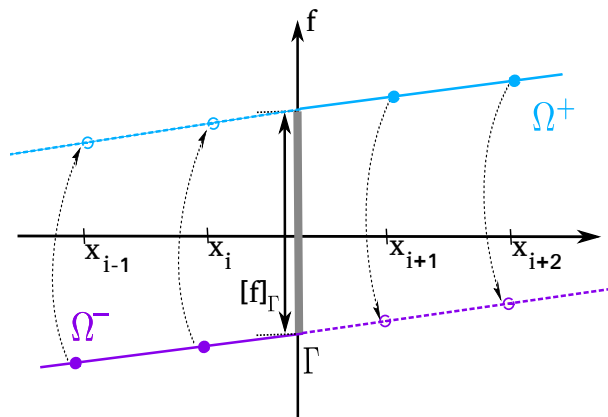
Figure 1.4: Schematics of the jump variable for Ghost Fluid method: real values (●) and ghost values (○).
