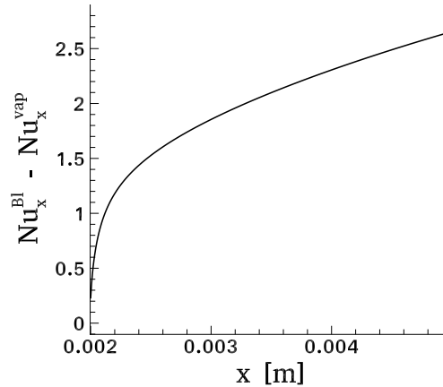
Fig. C.16. The correction on the Nusselt number from the Blasius theory with the x-axis - Vaporization configuration - dimensionless numbers: Pr = 1.022 , Re_{xL} = 85.726 , Ja = 3.69 and \frac{\rho_l}{\rho_v} = 17.746 .
