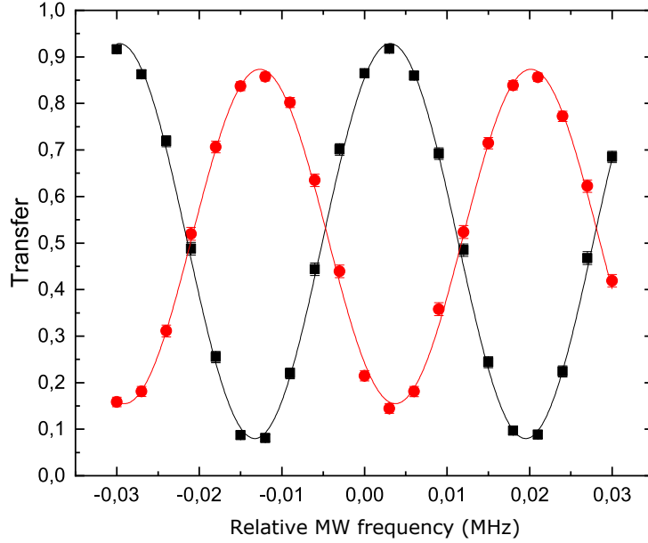
Figure 4.19: Ramsey fringes on the |51c\rangle \rightarrow |49c\rangle transition. Black data are taken in absence of the repumper pulses. Red data are taken in presence of repumper pulses. Solid lines are sinusoidal fits.
