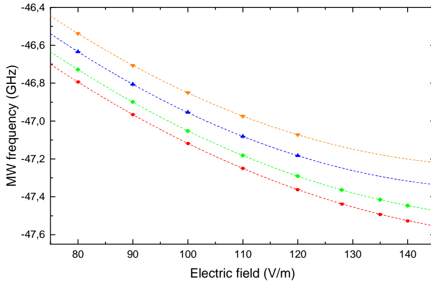
Figure 2.14: Energy difference between the |51^1G_4\rangle states and the |52^1F_3, m_{l_1} = +2\rangle state as a function of the electric field. The points are experimental data (red: |51^1G_4, m_{l_1} = +1\rangle , green: |51^1G_4, m_{l_1} = +2\rangle , blue: |51^1G_4, m_{l_1} = +3\rangle , orange: |51^1G_4, m_{l_1} = +4\rangle ), whereas the lines indicate parabolic fits. At 112.2 V/m, the energy difference between neighboring states is similar for all states from |m_{l_1} = +2\rangle on.
