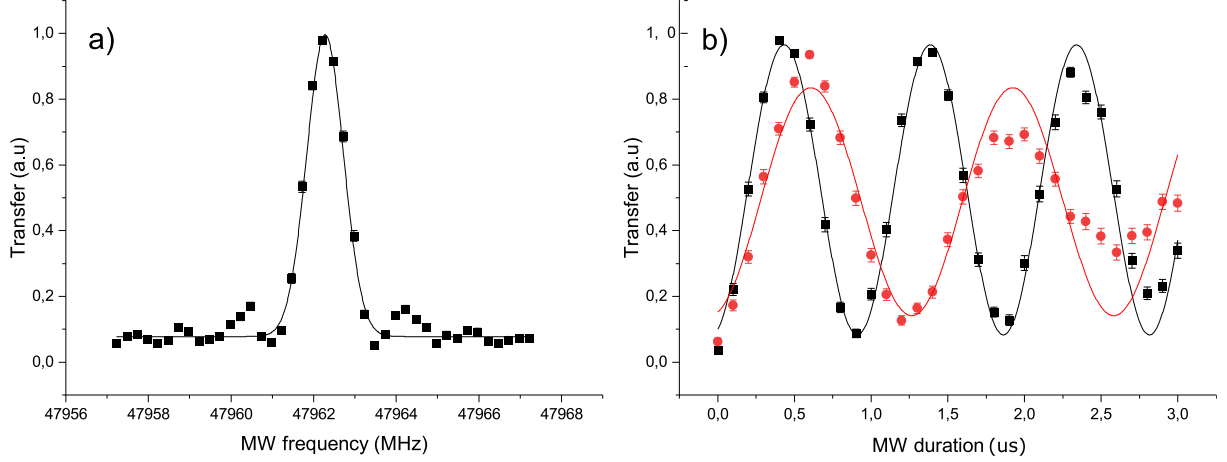
Figure 2.23: a) MW spectrum of the |51c\rangle \rightarrow |n = 52, n_1 = 0, m_{l_1} = 50\rangle transition (black squares). We set the MW frequency at \sim 47.962 GHz, i.e. the maximum of the transfer fitted by a Gaussian lineshape (solid line). b) Rabi experiments performed at the arrival time of the \pi/2 pulses of the Ramsey experiment. Black squares refer to the Rabi oscillations performed with the first MW pulse, red data to those performed with the second one. Solid lines are a guide for the eye.
