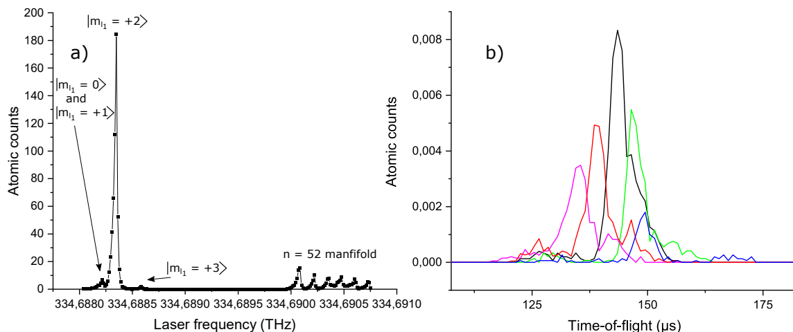
Figure 2.11: Laser spectrum of the Rydberg excitation to the |52^1F_3\rangle states. The highest peak represents the transition to the |52^1F_3, m_{l_1} = +2\rangle state. There are the |52^1F_3, m_{l_1} = 0\rangle , |52^1F_3, m_{l_1} = +1\rangle transitions on its left (unresolved by our laser) and the |52^1F_3, m_{l_1} = +3\rangle on the right. At very high frequency, we see the manifold of states with n = 52 . We lock the frequency of our laser at the top of the |52^1F_3, m_{l_1} = +2\rangle transition. The solid line is a guide for eye. b) Atomic counts as a function of the time-of-flight. We repeat the measurement for different Doppler corrections of the 896 nm laser frequency (black: 474 MHz, red: 479 MHz, green: 469 MHz, blue: 464 MHz, pink: 484 MHz). We set the Doppler correction in correspondence of the maximum atomic count recorded, centered upon a time of flight of (143.910 \pm 0.057) \mu\text{s} from the Rydberg excitation. The 461 nm and 767 nm laser frequencies are both kept locked throughout the measurement.
