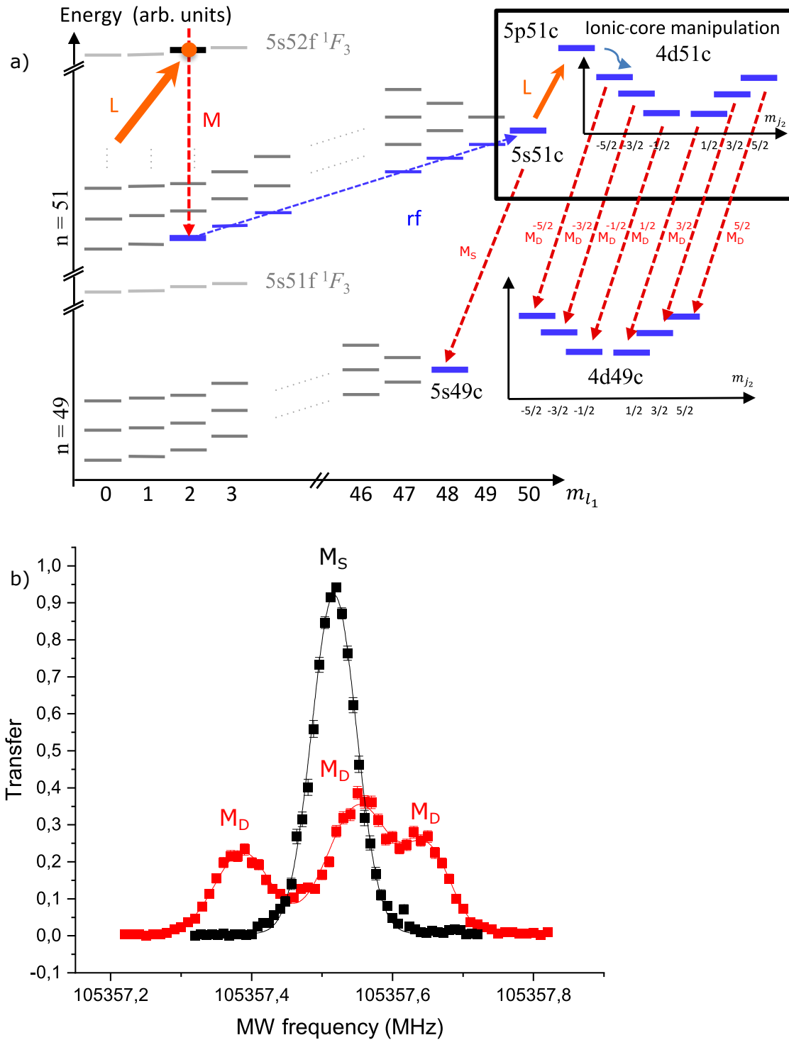
Figure 4.9: a) Navigation in the Hilbert space following our manipulations with rf, laser and MW pulses. b) MW spectra of the |51c\rangle \rightarrow |49c\rangle transition with (red data) and without (black data) the excitation of the core to the |4d_{5/2}\rangle states.
