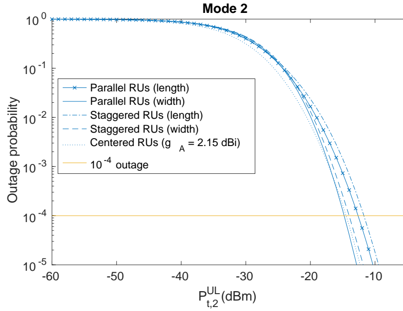
Figure 5.6: UL network outage with different RU placements for I = 4 .
