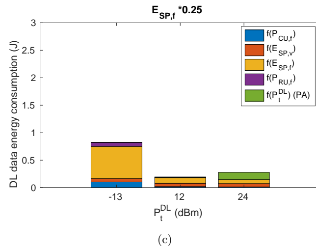
Figure 7.7: DL data transmission energy consumption.
