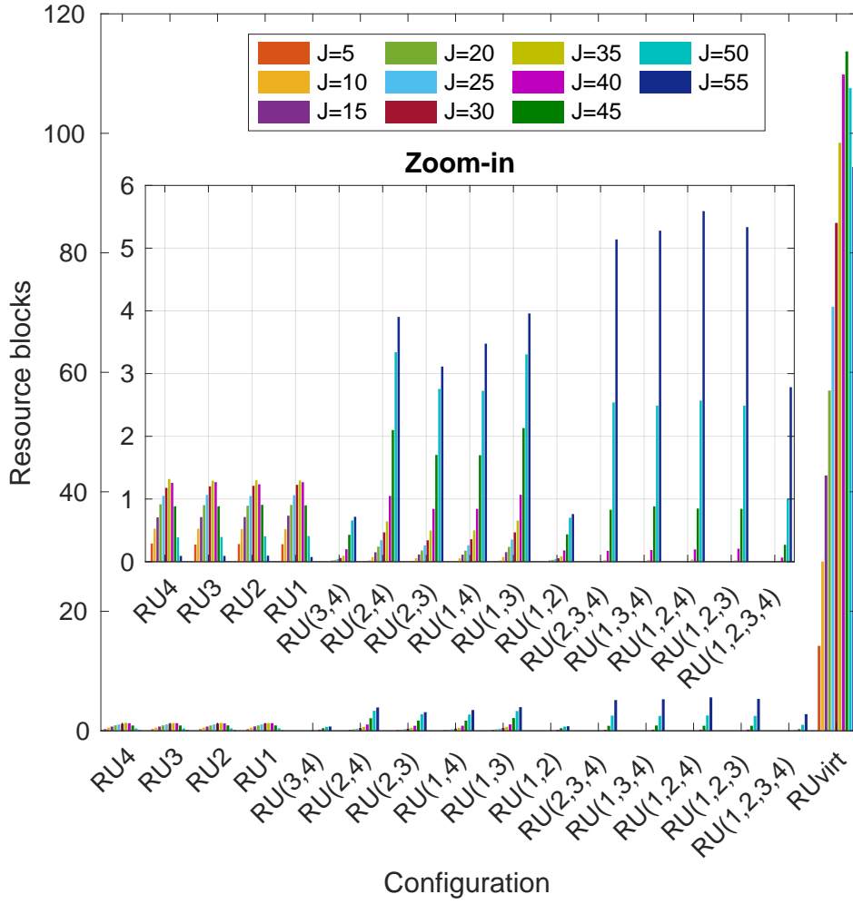
Figure C.2: Configurations usage for I = 4 with virtual RU.
