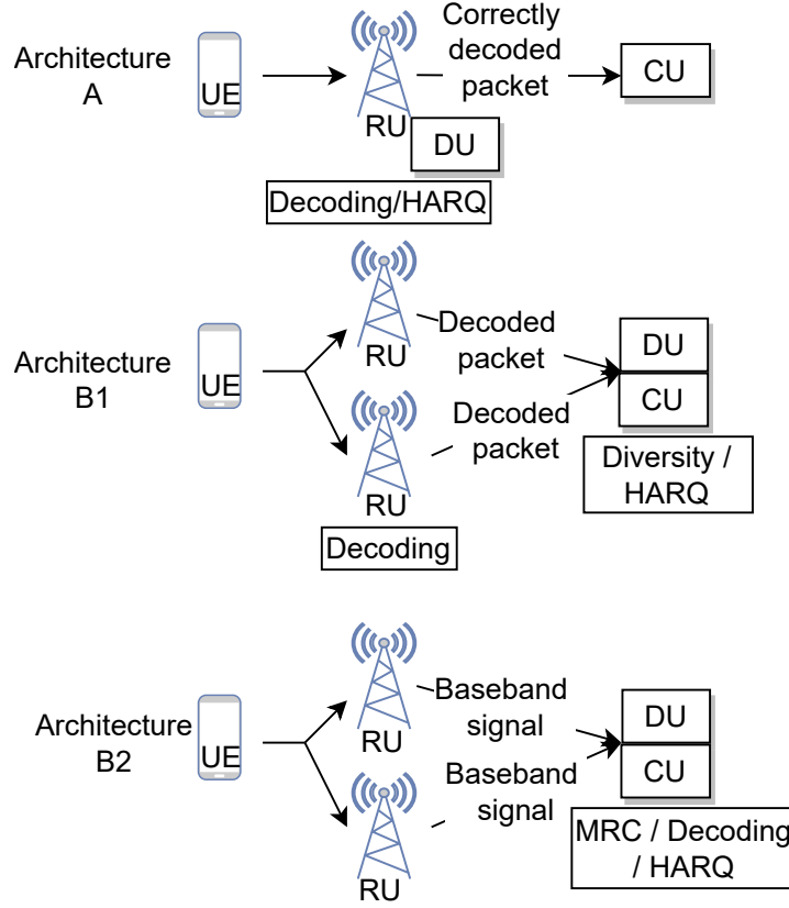
Figure 4.1: Architectures A, B1, and B2.
