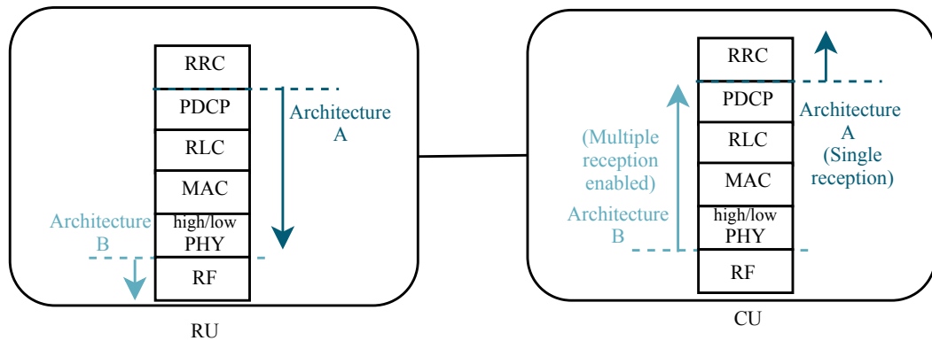
Figure 3.8: Flexible split.
