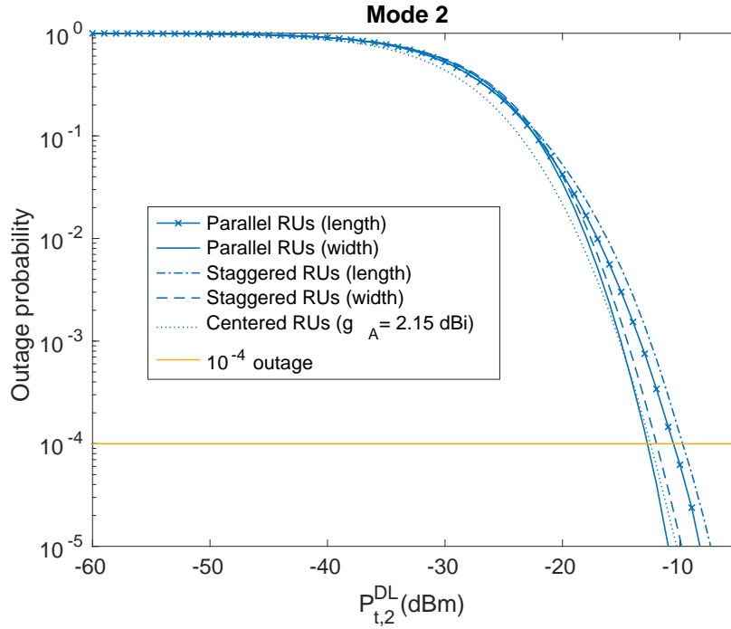
Figure 5.5: DL network outage with different RU placements for I = 4 .
