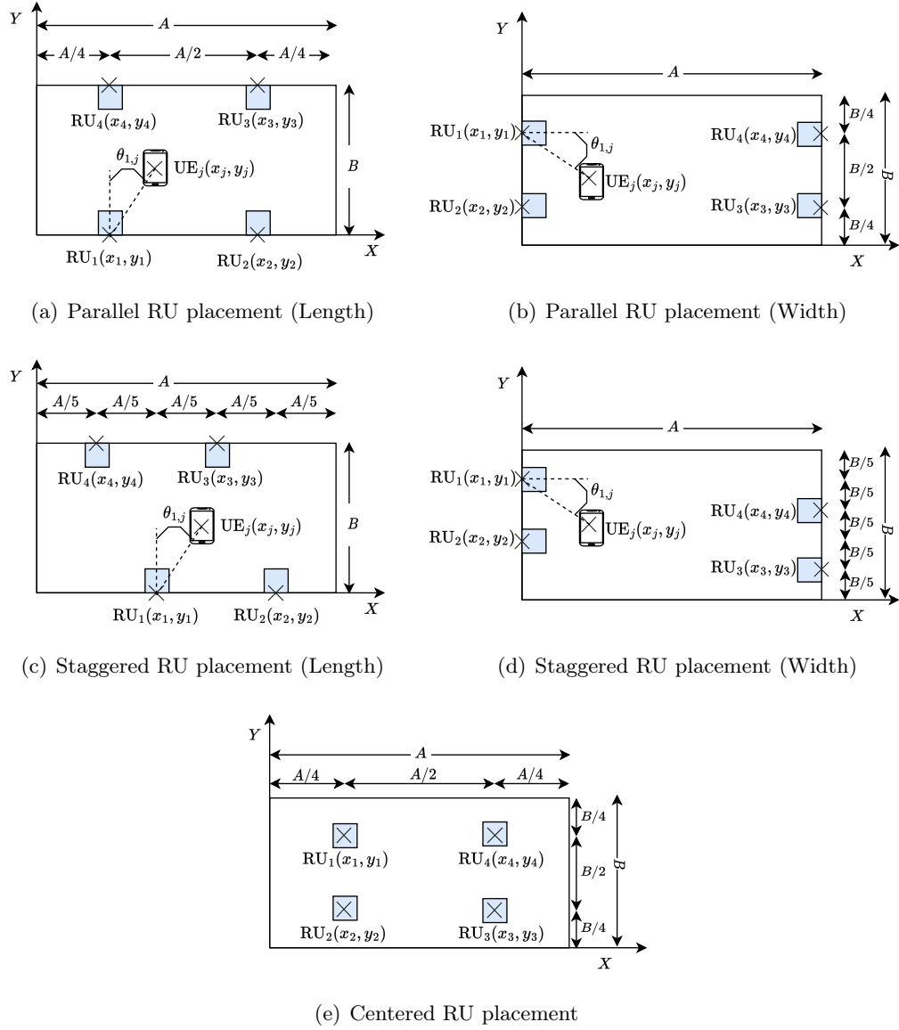
Figure 5.4: RU placement for I = 4 .
