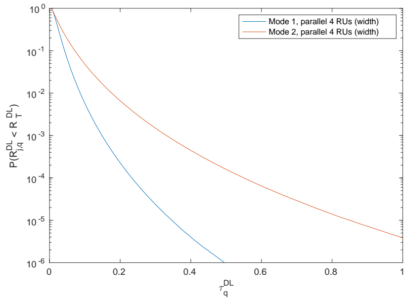
(a) Downlink
