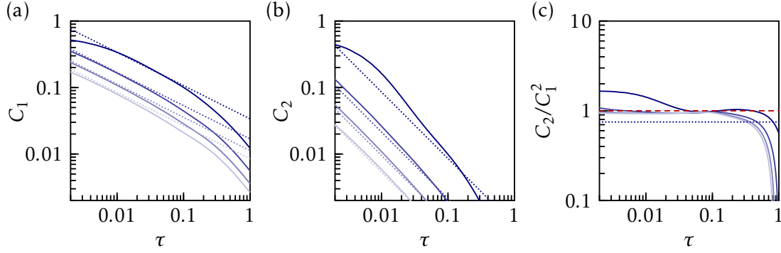
Figure 4.2 Numerical solutions of (a) C_1(\tau) , (b) C_2(\tau) and (c) C_2(\tau)/C_1^2(\tau) , using equation (4.3.13) and equation (4.3.14) with U/J = 10 and \epsilon = 0.01 . We vary the filling \bar{n} : from darker to brighter lines, \bar{n} = 2, 4, 6 and 8 . The dotted lines correspond to the large filling limit. In (c), the dashed line corresponds to C_2/C_1^2 = 1 .
