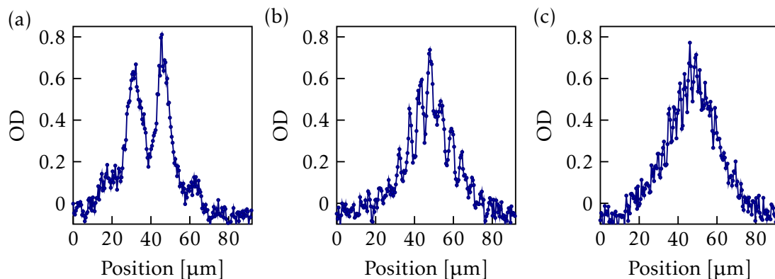
Figure 6.3 Cut of in-situ images of the atoms trapped by the LPL and a lattice of period (a) 15 \mu\text{m} , (b) 6 \mu\text{m} and (c) 3 \mu\text{m} .
