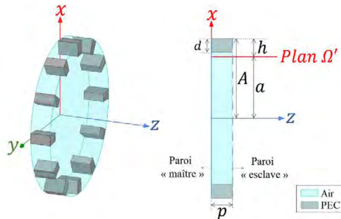
Figure 4.17 - Cellule élémentaire HFSS.
