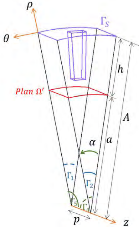
Figure 4.3 – Cellule élémentaire 3-D.
