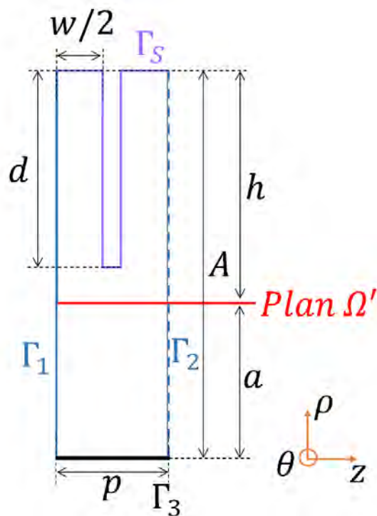
Figure 3.19 – Cellule élémentaire de la corrugation, avec A = 34.2 mm, a = 13.68 mm, d = 17.4 mm, h = 20.52 mm, p = 11.5 mm, et w = 8.5 mm.
