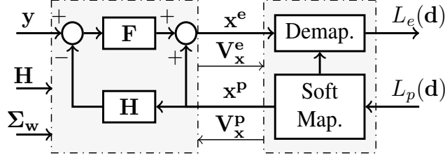
Figure 2.4: Turbo receiver based on the generic linear MMSE SISO detector.
