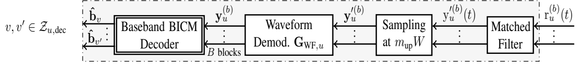
Figure 1.6: Block diagram of a single carrier receiver.
