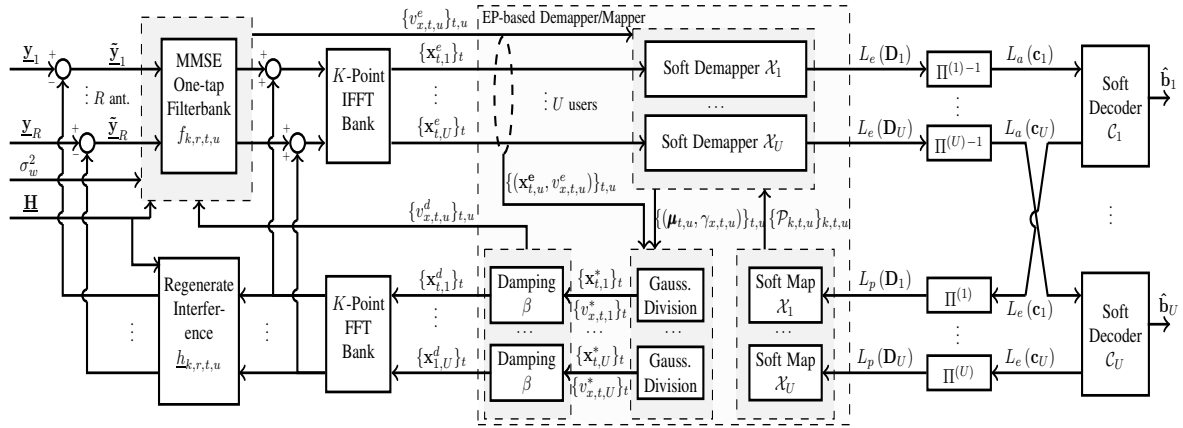
Figure 4.27: Proposed iterative MU-MIMO SC-FDMA receiver with bin-wise filterbank and interference cancellation based on EP.
