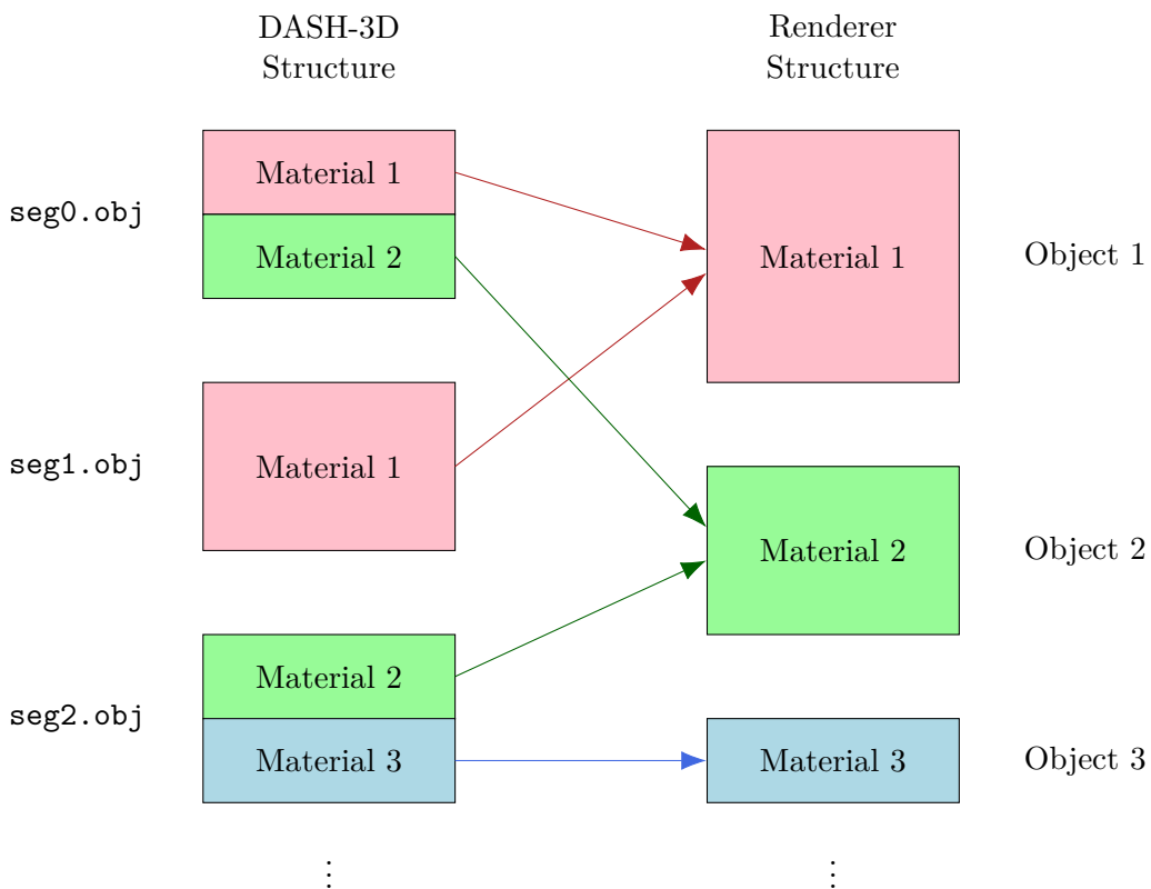
Figure 4.4: Reordering of the content on the renderer
