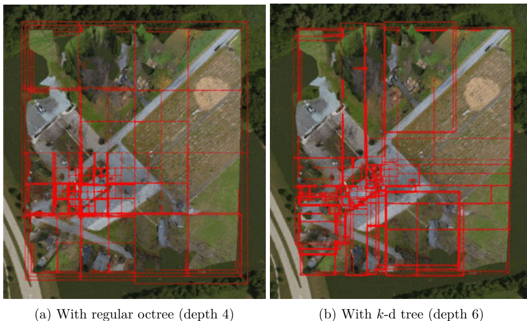
Figure 2.6: Spatial partitioning used in 3D Tiles
