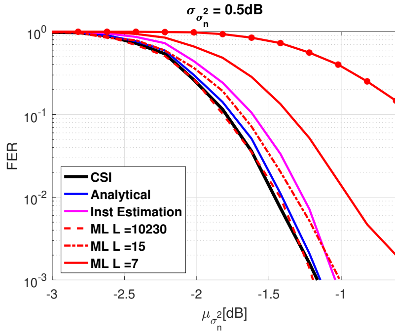
Figure 5.2: GPS L1C subframe2 Frame Error Rate Considering a Smoothly Variation of the Variance \sigma_n^2 within the Codeword.
