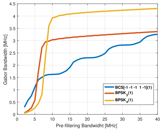
Figure 2.21: Gabor bandwidth of the candidate signals.
