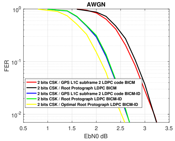
Figure M.9: FER under BICM-ID scheme M = 2
