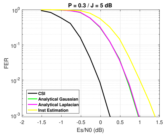
Figure 5.25: GPS L1C FER under a Pulsed Jamming/ P = 0.3 and J = 5dB
