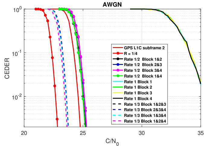
Figure 4.29: CEDER over AWGN Channel considering: the irregular LDPC code of GPS L1C subframe 2 (red/solid line); the rate compatible Root LDPC code of rate 1/4 when the entire codeword has been received (red/solid-dash line); the rate compatible Root LDPC code of rate 1/4 when one data block unit has been received (cyan/solid line 1-st block; green/solid line 2-nd block; yellow/solid line 3-rd block; black/solid line 4-th block); the rate compatible Root LDPC code of rate 1/4 when two data block units have been received (black/solid-point line 1-st and 2-nd blocks; blue/solid-point line 2-nd and 3-rd blocks; magenta/solid-point line 3-rd and 4-th blocks; green/solid-point line 1-st and 4-th blocks); the rate compatible Root LDPC code of rate 1/3 when three data block units have been received (black/dash line 1-st to 3-rd blocks; blue/dash line 2-nd and 4-th blocks; cyan/dash line 1-st, 3-rd and 4-th blocks; magenta/dash line 1-st, 2-nd and 4-th blocks).
