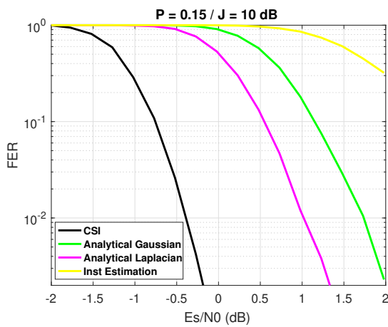
Figure 5.12: GPS L1C FER under a Pulsed Jamming/ P = 0.15 and J = 10dB
