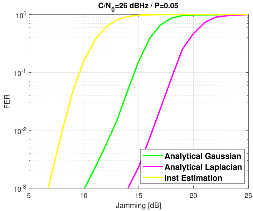
Figure 5.32: GPS L1C subframe 2 FER C/N_0 = 26dBHz with P = 0.05
