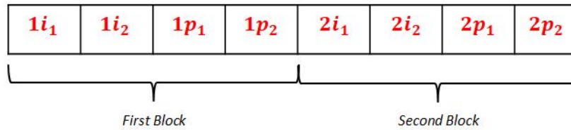
Figure 4.39: Channel model for the unequal error protection Root LDPC codes.
