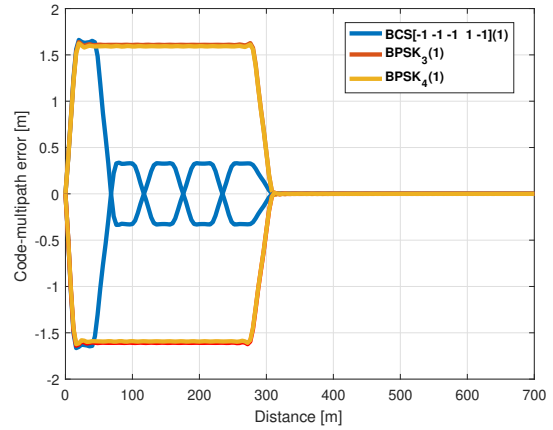
Figure 2.20: MPEE of the candidate signals.
