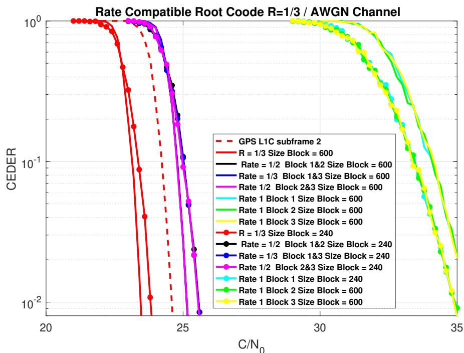
Figure I.1: Retrieved CED error rate over AWGN channel with different CED block sizes and codes of rate R = 1/3 .
