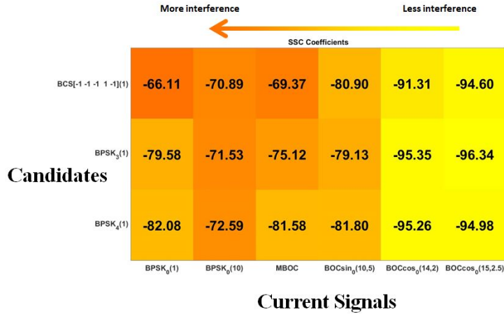
Figure 2.18: SSC between Legacy and proposed signals
