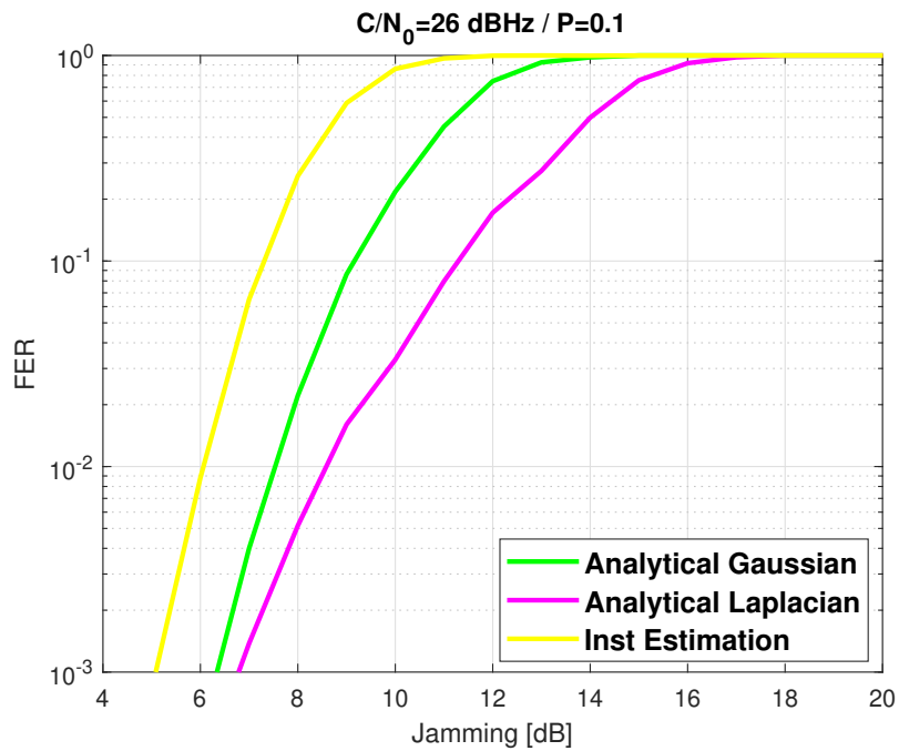
Figure 5.33: GPS L1C subframe 2 FER C/N_0 = 26dBHz with P = 0.1
