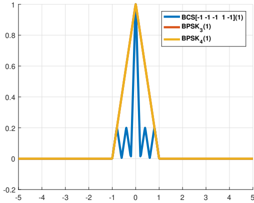
Figure 2.19: ACF of the candidate signals.
