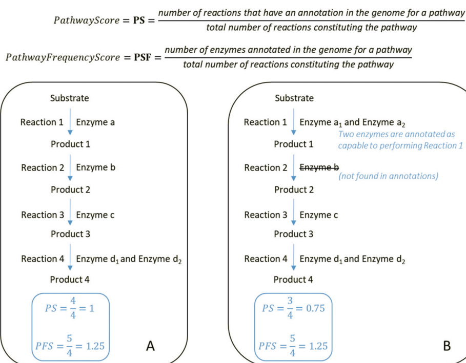
Figure 2. At the top, formulas for the computation of the PS and PFS. Below, examples of two types of computations of the PS and PFS based on an example of a hypothetical metabolic pathway. By comparing the PS and PFS in A and B , pathway A shows greater evidence of its veracity.
