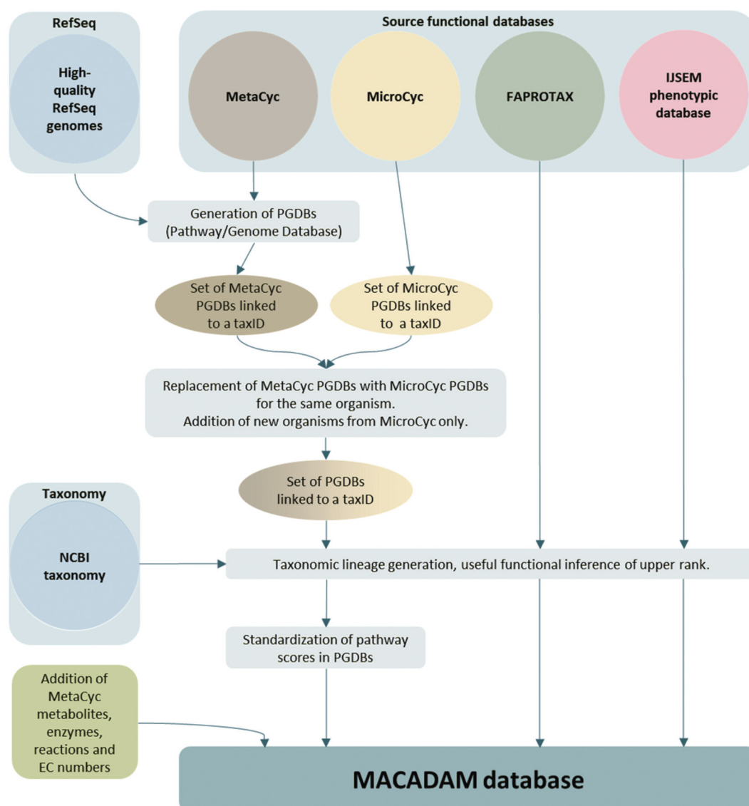
Figure 1. MACADAM building workflow.
