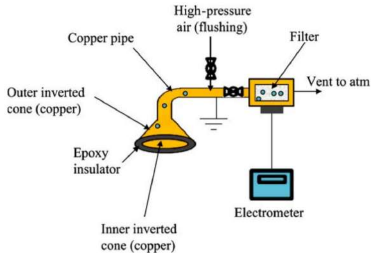
Figure 1.10: Sampling device of Fotovat et al. 2016
