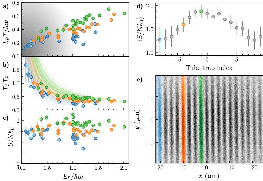
Figure 5.8: Thermodynamics of the 1D-3D crossover. The data points in a), b), c) and d) represent the local quantities at the center of the trap ( z = 0 ) where the local Fermi energy is the highest, and the colors indicate the selected tubes, shown in e). a) Temperature normalized by the transverse quantum of energy \hbar\omega_{\perp} . The grey gradient illustrates the 1D region. b) Temperature normalized by the Fermi temperature. The solid lines emanating from the data points represent the continuous change in E_F/\hbar\omega_{\perp} and T/T_F within each atomic wire according to LDA. c) Normalized entropy per particle. d) Mean value of the entropy per particle obtained by averaging the data of c) for the green, orange, and blue points. The grey points represent the other 15 tubes traps which were omitted in a), b) and c). e) Optical density obtained from a characteristics absorption image. The colour code indicates the selected tubes.
