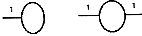
Figure 4.24: Two graphs of genus 1
