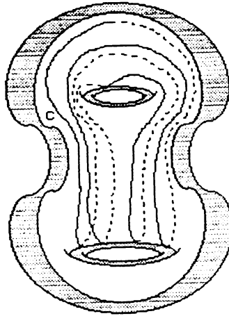
Figure 4.43: R_2 and the attaching curve c
