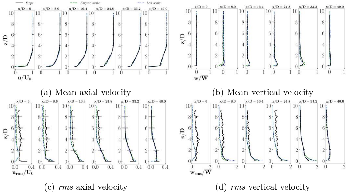
Figure 7.12: Time-averaged velocities with upstream turbulence.
