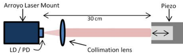
Figure 2.3: Experimental setup. Piezo modulated at two separate frequencies.
