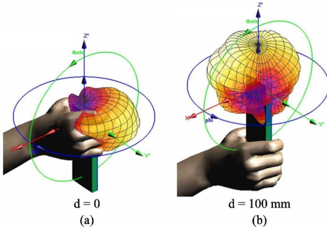
Figure 2.6: Simulated 3D Radiation Pattern of a Smartphone Antenna in hand-held Conditions at 1795 MHz. a) d = 0 mm. b) d = 100 mm. Figure taken from [5]
