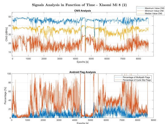
Figure C.2: Signal Analysis of the Xiaomi Mi8 (2). a) Upper Figure: C/N0 Analysis. b) Lower Figure: Percentage of Android Flags Activation
