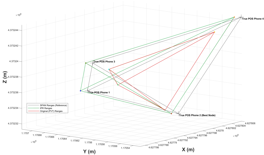
Figure 6.3: Inter-Phone Range Vector ( \mathbf{IPR}_{3D} ) Constraint Visualization in 3D - ECEF Coordinates in [m]
