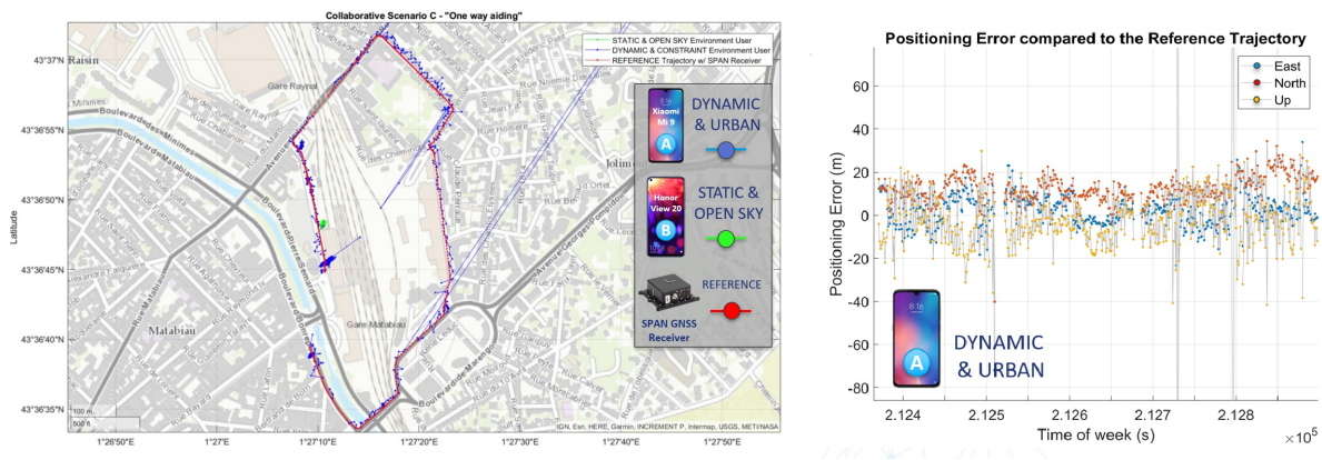
Figure 3.20: Smartphone FLP Positioning Solutions Compared to Reference Trajectory during Collaborative Scenario C and the Associated Smartphone Positioning Error Analysis in [m]
