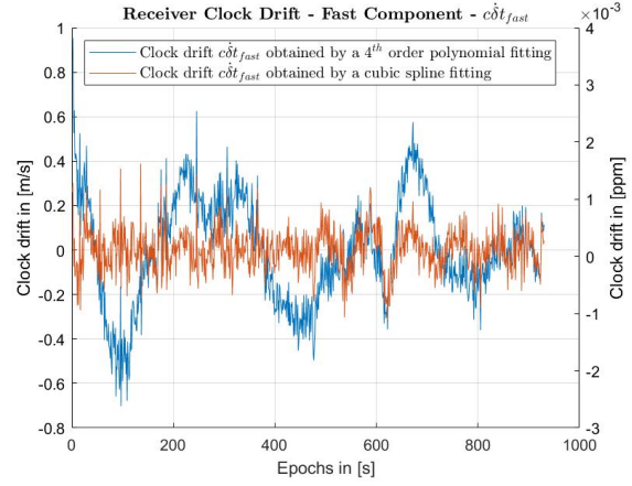
Figure 3.11: Clock Drift Fast Component ( \dot{c}t^{fast} )
