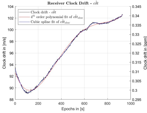
Figure 3.10: Receiver Clock Drift in [m/s] and [ppm] ( \dot{c}t )
