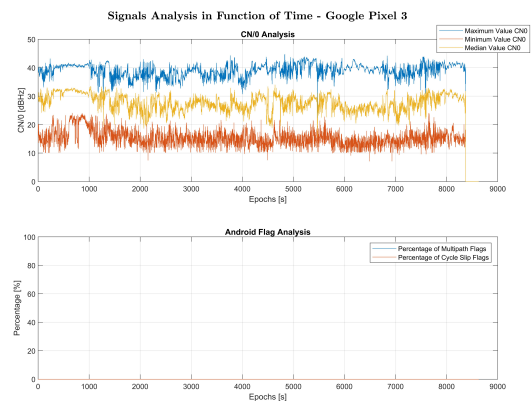
Figure C.6: Signal Analysis of the Google Pixel 3. a) Upper Figure: C/N0 Analysis. b) Lower Figure: Percentage of Android Flags Activation
