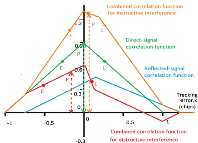
Figure B.4: Effect of Multipath Interferences on the Correlation Function for both Constructive and Distructive Effects. Pictured extracted from [18]
