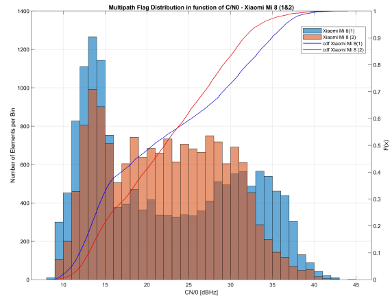
Figure 3.24: Multipath Android Flags Detection Histogram Distribution for the two Xiaomi Mi 8
