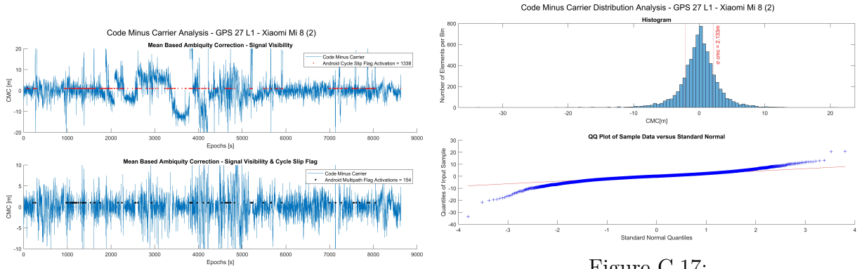
Figure C.16: Code-Minus-Carrier Correlation Analysis for the Xiaomi Mi8 (2) - GPS PRN 27 L1
