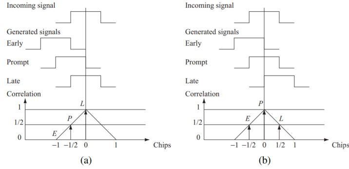
Figure A.8: Code Delay Tracking. (a) Signal Synchronization not Achieved. (b) Perfect Code Tracking. [17]
