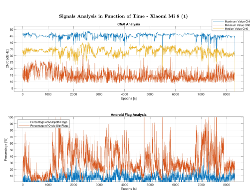
Figure C.1: Signal Analysis of the Xiaomi Mi8 (1). a) Upper Figure: C/N0 Analysis. b) Lower Figure: Percentage of Android Flags Activation
