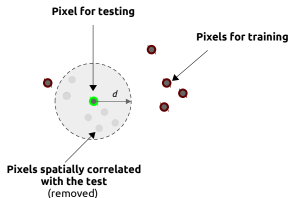
FIGURE 2.4 – Spatial leave-one-out cross-validation (SLOO-CV) schema for one class. One pixel is used for testing. The other pixels are used for training, except pixels geographically too close to the pixel selected for testing. This procedure is repeated n times where n is the number of reference samples. Spatial autocorrelation between nearby pixels is assumed up to a distance d which can be estimated using Moran's I.
