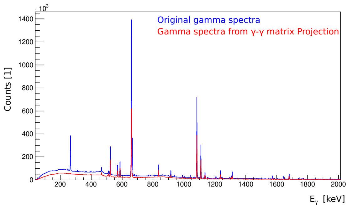
Figure 3.20 – Comparison between projection spectrum from Figure 3.19 and the original spectrum from HPGe detectors.
