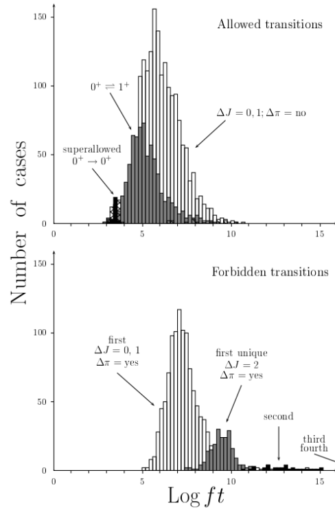
Figure 1.7 – A summary of \log ft values from [21].
