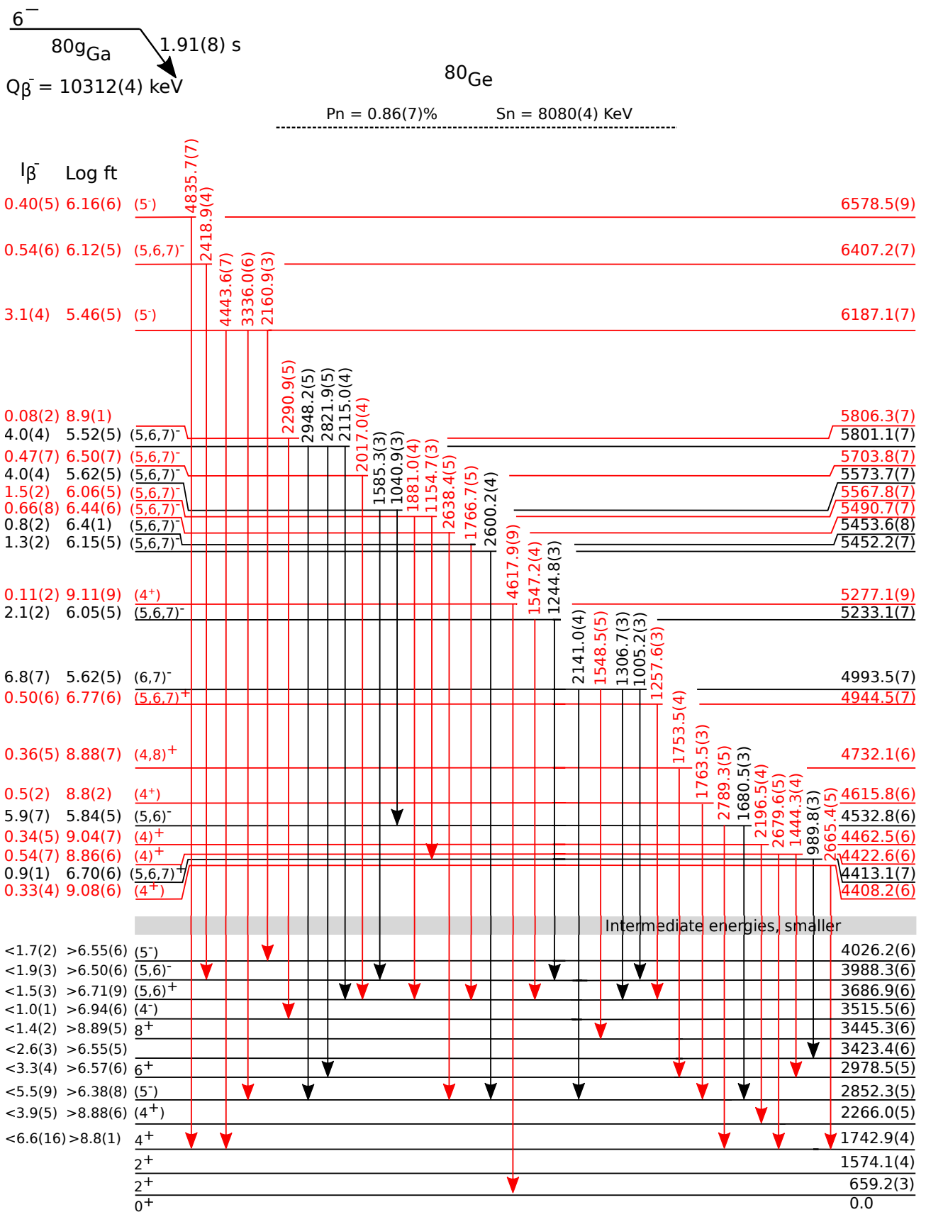
Figure 4.18 – Level scheme of ^{80}\text{Ge} populated following the \beta -decay of ^{80g}\text{Ga} ( 6^- ) containing the high-lying states between 4.2 and 8 MeV in energy.
