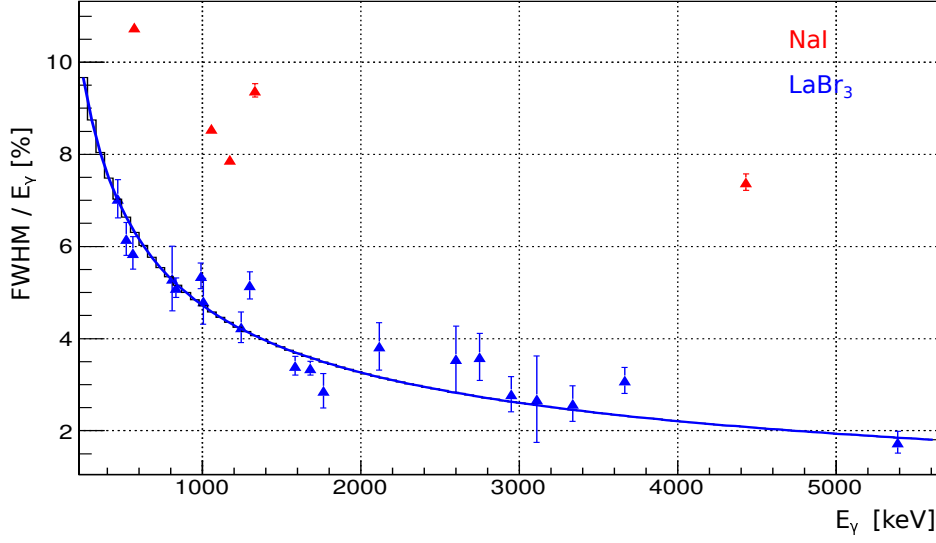
Figure 3.15 – Energy resolution as a function of the \gamma -ray energy of the individual LaBr 3 and NaI components of the PARIS phoswich detectors. Fitting function used is \text{FWHM}/E_\gamma = a(E+bE^2)^{-1/2} .
