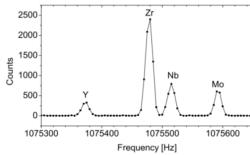
Figure 1.23 – A quadrupole frequency scan in the JYFLTRAP purification trap for mass A = 100 in which each point is accumulated for 50 cycles and the spectrum was plotted with collection of 30 min [83].
