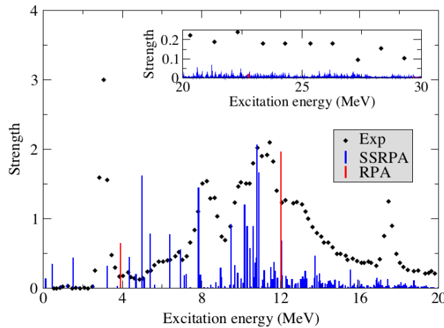
Figure 1.4 – B(\text{GT}) distributions for ^{48}\text{Ca} of experiment \text{MeV}^{-1} (black points), RPA and SSRPA calculations. Notice: to better display the results, the RPA and SSRPA strengths were rescaled as RPA strength was divided by nine and multiply the SSRPA strength by two [17].
