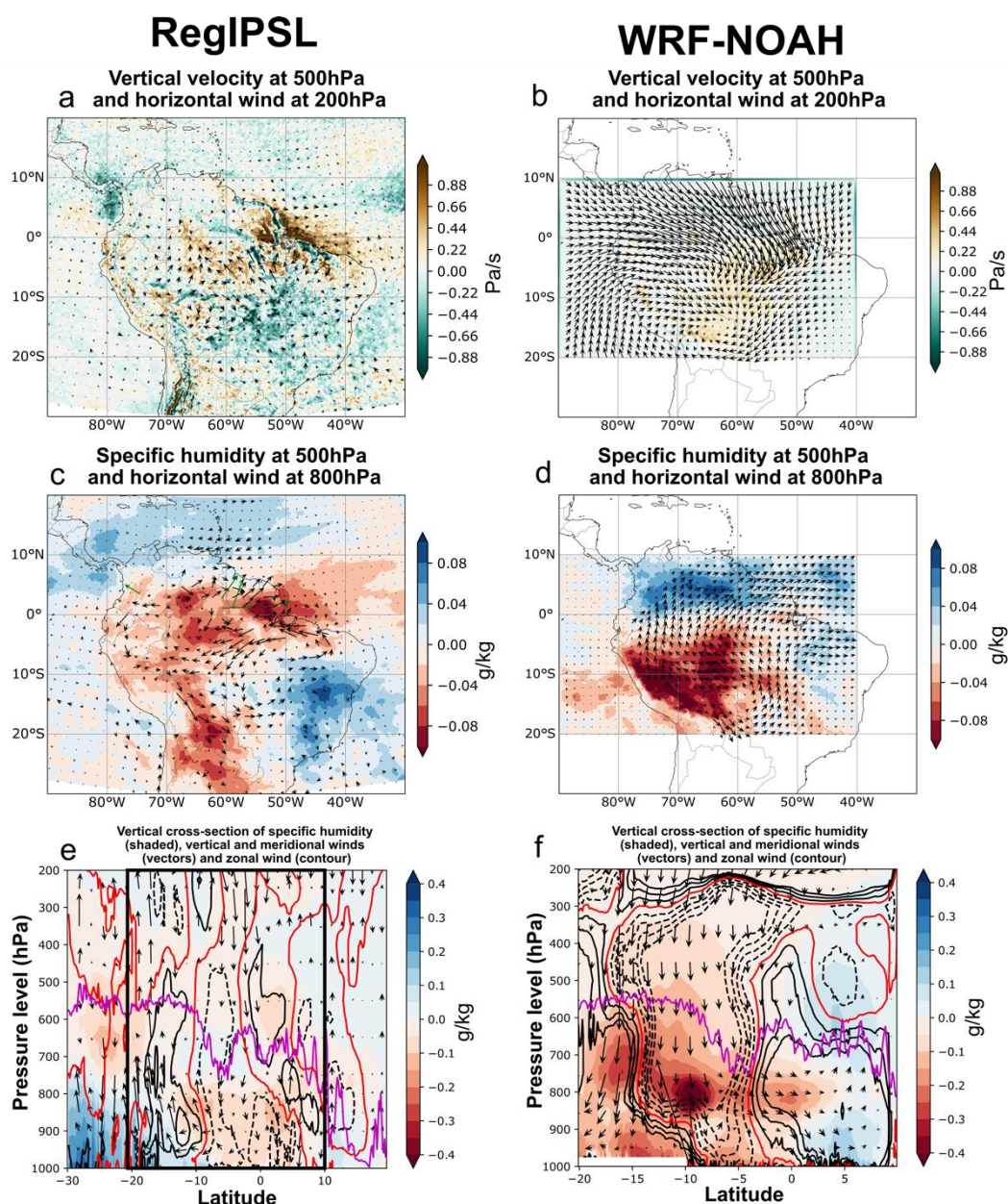
Fig. 5.8 December-February climatological differences Deforested minus Control for RegIPSL ( a-c-e ) and WRF-NOAH ( b-d-f ): a-b 500 hPa (vertical velocity shaded, units in \text{Pa s}^{-1} ) multiplied by a factor of 100 and 200 hPa horizontal winds (vectors, units in \text{m s}^{-1} ), c-d 500 hPa specific humidity (shaded, units in \text{g kg}^{-1} ) and 800 hPa horizontal winds (vectors, in \text{m s}^{-1} ), d-e pressure-latitude cross-section of the zonally-mean meridional circulation in the tropical North Atlantic and western South America. Zonal-Mean is calculated over a region encompassing the easternmost side of the 3000 m elevation contour and the 60^\circ\text{W} . Meridional and vertical (multiplied by a factor of 100) components of the winds for vectors (in \text{m s}^{-1} and \text{Pa s}^{-1} , respectively), specific humidity (shaded, units in \text{g kg}^{-1} ) and zonal wind in contour (solid lines represent positive/westerly winds and dashed lines represent negative/easterly winds; the red line shows the 0 \text{ m s}^{-1} contour). Magenta line in e-f shows the Andes' profile calculated as maximum orographic elevation in the Andes axis. The black rectangle in e represents the area shown in f .
