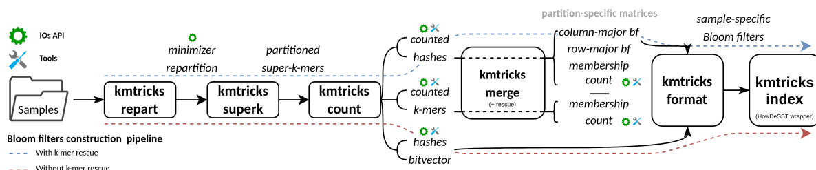
Figure V.1 – Overview of kmtricks modules. The blue and red arrows correspond to the BF construction pipeline with or without k -mer rescue, respectively.
