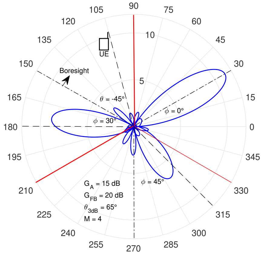
Figure 2.3 – Radiation pattern of tri-sectored BS capable of performing beamforming
