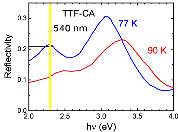
Figure 3.24: Comparison of reflectivity spectra measured perpendicular to \vec{a} axis in both Neutral Paraelectric phase (red) and Ionic Ferroelectric phase (blue). The selected probe energy (2.3 eV) appears in Yellow. Figure adapted from [Dressel and Peterseim, 2017]
