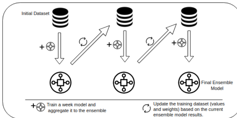
Figure A.7: Boosting process
