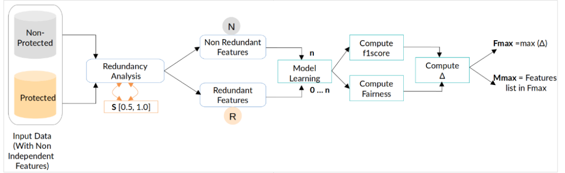
Figure 4.1: The proposed approach and its different stages
