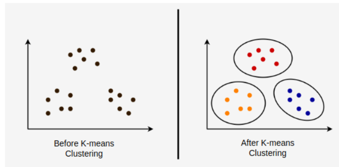
Figure A.8: An example of K-means clustering
