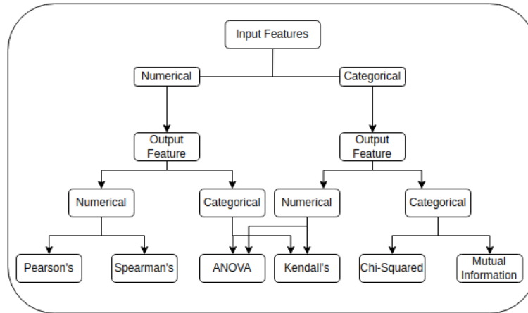
Figure 2.8: Statistical tests for Filter selection method [Jović et al. , 2015]
