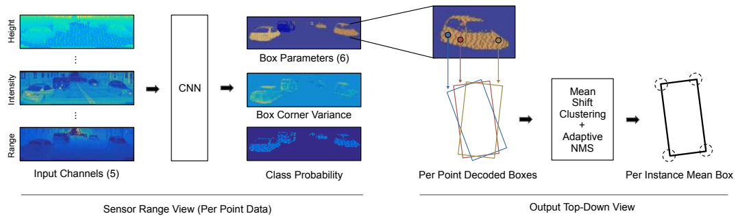
FIGURE 2.18: Architecture of LaserNet method proposed by Meyer et al. [55, Fig. 2].
