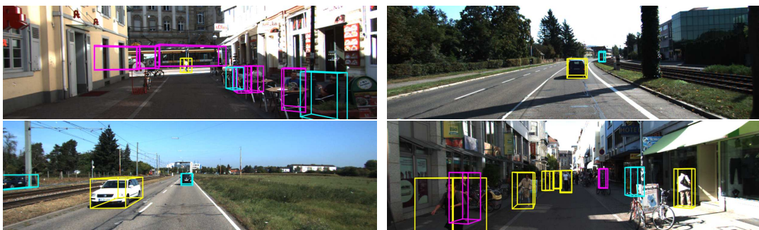
FIGURE 3.6: Example of the difficulty level of the objects in the KITTI dataset corresponding to the definition in Table 3.3. Easy, Moderate and Hard objects are shown in yellow, blue and pink 3D bounding boxes.
