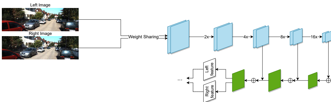
FIGURE 5.7: Modified feature extraction part of the SLS-Fusion algorithm to adapt it for taking only the stereo camera as input.
