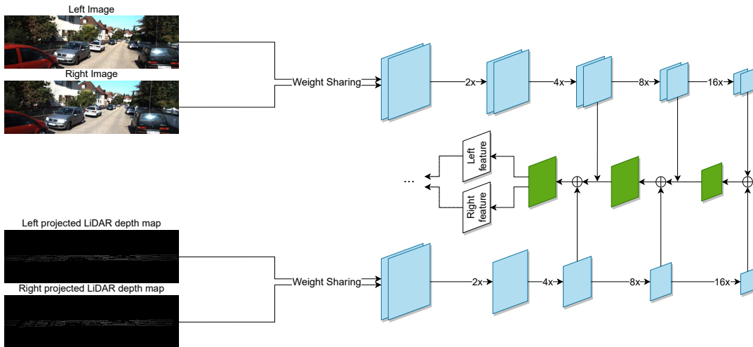
FIGURE 5.6: SLS-Fusion feature extraction part. It takes both images and point cloud as input.
