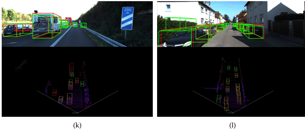
FIGURE 4.9: Qualitative Comparison. We illustrate the results of SLS-Fusion with different input point clouds on a KITTI validation scene. They are visualized in a frontal-view image as well as a BEV point map. Ground-truth and predicted boxes are in red and green, respectively.
