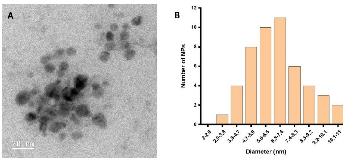
Figure S 3.7. TEM images and size distribution of the AuNPs*.
