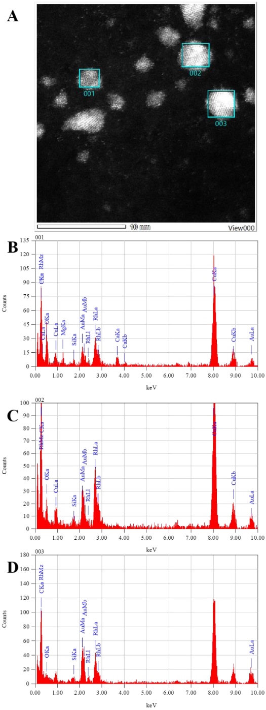
Figure S 2.12. HRTEM-EDX image of Au 1 Rh 2 NZs (A), element distribution of 001 area (B), 002 area (C) and 003
