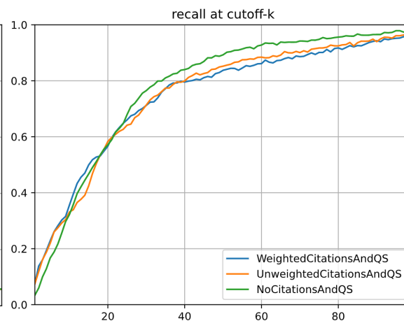
Figure 6.9: Average recall at cutoff-k.
