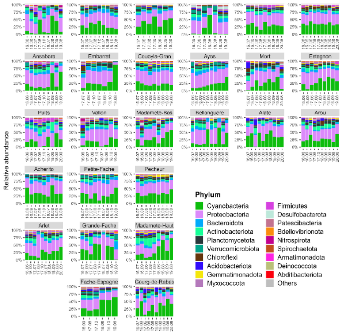
Figure 20: Composition bar plot (relative abundance) of the prokaryotic biofilm assemblages (determined by metabarcoding of the 16S rRNA gene) of the 231 biofilm samples sequenced in this study, represented at the Phylum level. Each facet is a lake with all its sample (sorted in chronological order: dates on the x-axis, 16.06 means June 2016), and each column contains all the lakes of a same gradient, sorted by increasing elevation (top = lowest). The 19 most abundant phyla were selected with this plot (the 25 others are grouped in the category “Others”). Phyla are sorted by total abundance from bottom to top of each barplot, with legends arranged accordingly.
