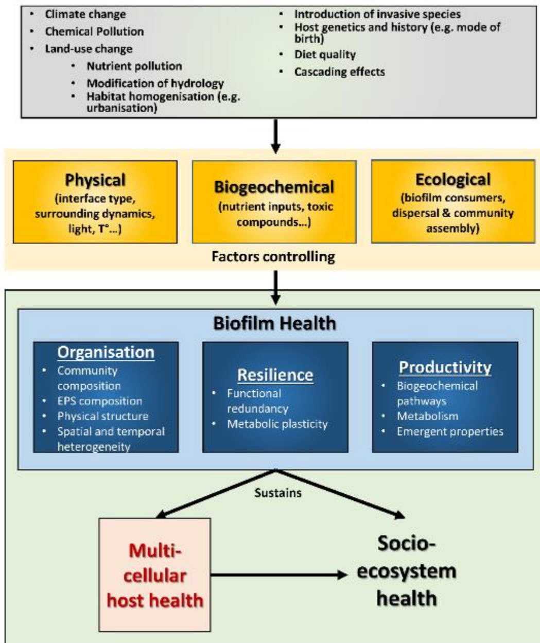
Figure 11: Factors controlling biofilm health. A: broad range of physical, biogeochemical and ecological factors (yellow box) can drive biofilm health and have further implications on the system where biofilms occur (green box; see also Figure 12 and Figure 13 ). These factors are themselves impacted by drivers of global environmental change and/or host-related factors (grey box).
