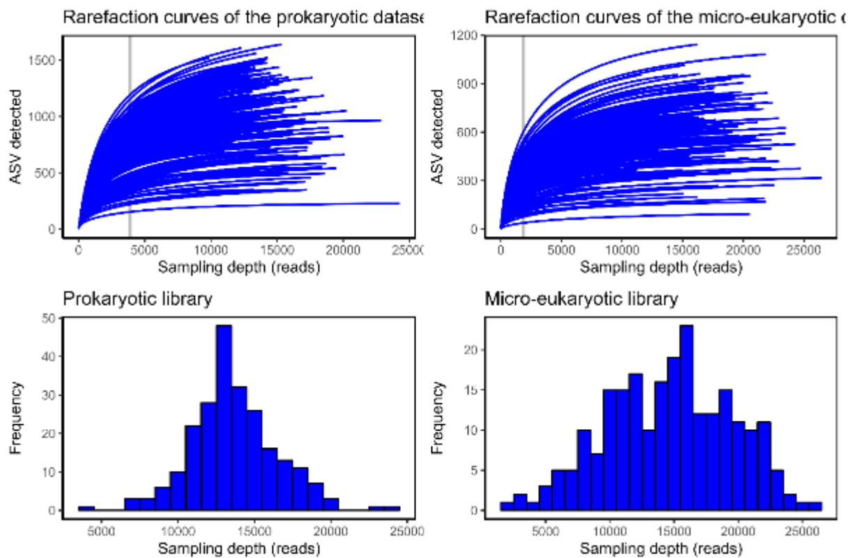
Figure 18: Rarefaction curves (upper) and histograms (lower) of the prokaryotic and micro-eukaryotic datasets (left and right respectively). Grey vertical lines indicate the depth used for rarefaction (3897 and 1856 reads, respectively). Four and six samples, inferior to the thresholds, were discarded.
