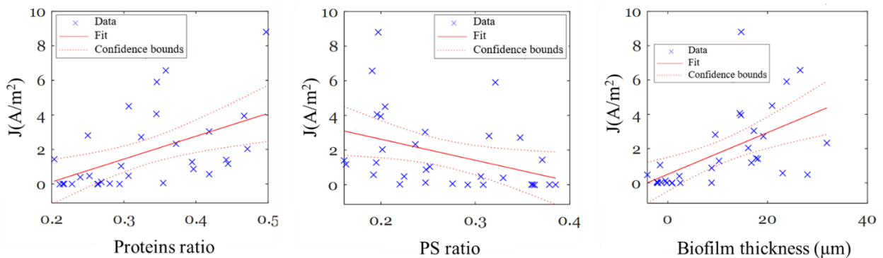
Figure V-19 : Scattered plots of significant EPS components on current density for tests 5.3, 5.4, 5.5 and 5.6. PS: \alpha -polysaccharides.
