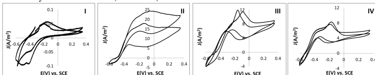
Figure S3. Cyclic voltammeteries for duplicate experiments performed at 1 mV/s at the end of each stage without adjusting the y-axis scale.
