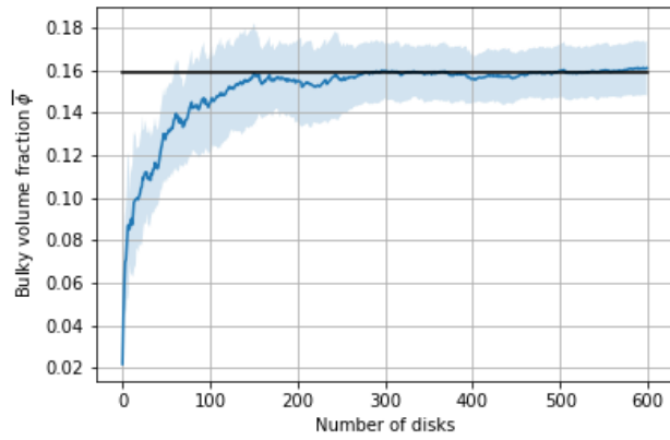
Figure 2.30: Convergence of the bulky volume fraction with the number of disks (diameter of 10mm) for 20 random realizations on a domain of 100mm. The average value over the realizations (continuous blue line) is compared with the theoretical value given by the stack description (black line). The blue envelope gives the interval +/- the standard deviation around the average value.
