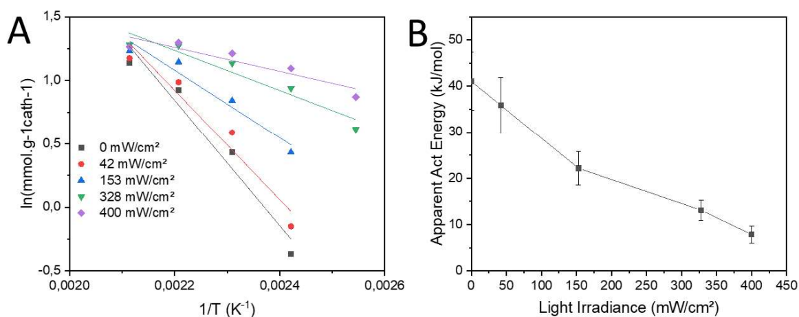
Fig. 90 (A) Arrhenius plot for the methane yield obtained over the Ru(5%)/TiO 2 (PA) catalyst and (B) Light-dependency of the apparent activation energy of CO 2 conversion to CH 4 . Reaction conditions: [CO 2 ] = 2000 ppm v , [H 2 ] = 8000 ppm v , total Ar flow of 5.8 mL/min, 5.0 mg of catalyst, CO 2 specific molar rate of 5.7 mmol g -1 h -1 .
