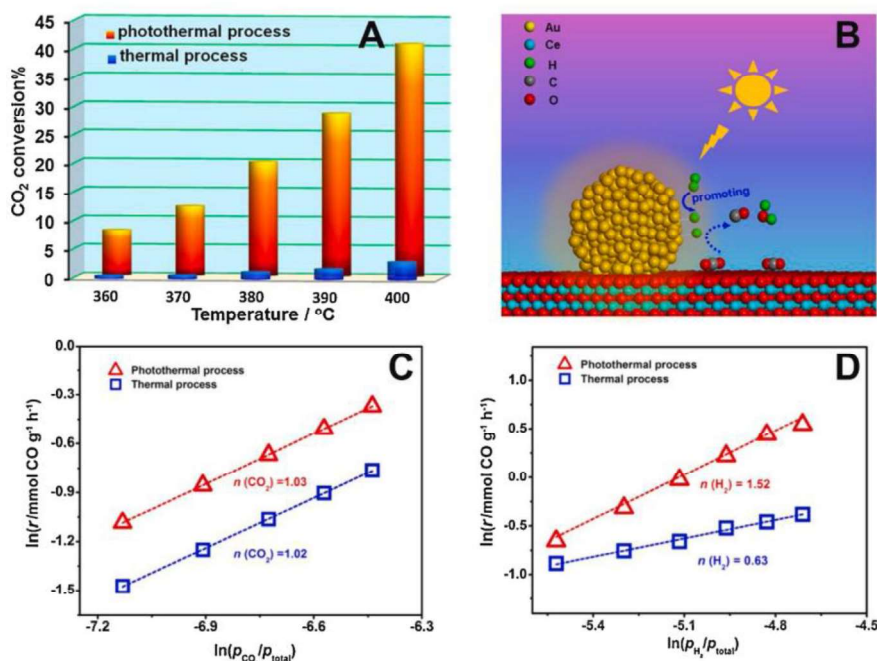
Fig. 22 A) \text{CO}_2 conversion values in RWGS reaction over 0.9 at. % Au/CeO 2 from 360- 400 °C in the dark (blue) and under illumination (red) conditions. B) Mechanistic scheme showing the promotion of H 2 dissociation over Au atoms. C) Plot of CO production rate dependence on partial pressure of CO 2 in the dark and under illumination, and D) on partial pressure of H 2 . (reproduced from ref. [150])
