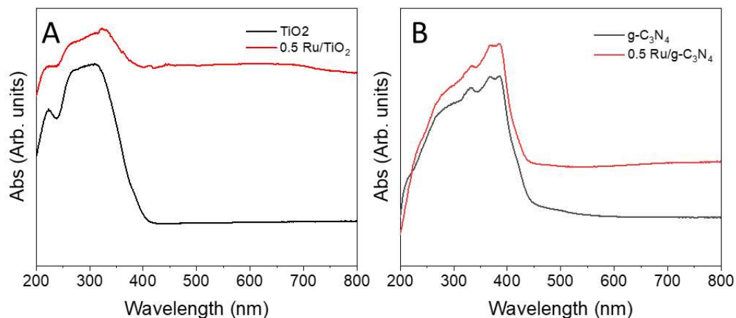
Fig. 66 UV-Vis spectra of the bare \text{TiO}_2 and g\text{-C}_3\text{N}_4 supports, and of both \text{Ru}/\text{TiO}_2 and \text{Ru}/g\text{-C}_3\text{N}_4 catalysts.
