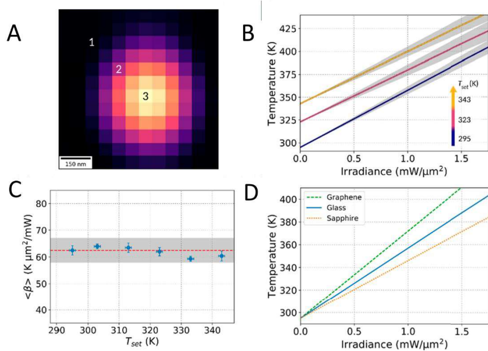
Fig. 8 PL-AS nanothermometry applied to gold single particle under green laser irradiation results where a) is the hyperspectral image of a single Au nanoparticle, b) photon irradiance dependance of the local temperature at different (global) temperatures, c) photothermal coefficient values at different set temperatures, and d) influence of the underlying substrate on the dependance of the local temperature with the irradiance (Figure adapted from ref [79])
