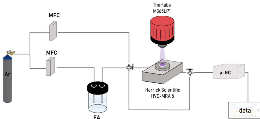
Fig. 27 Scheme of the photo thermal catalytic set up for FA conversion.
