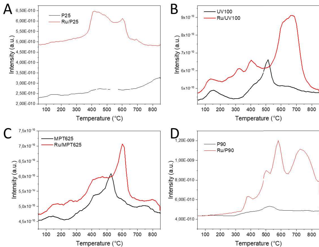
Fig. A 2 CO 2 -TPD graphs of the m/z =28 signal of bare TiO 2 supports (black) and supported Ru (red) on A) P25, B) UV100, C) MPT625 and D) P90.
