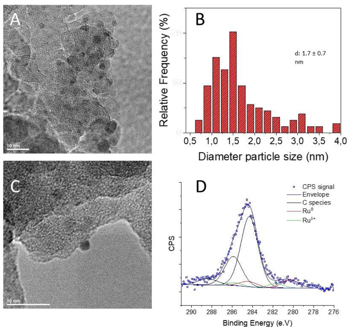
Fig. 64 Characterization of the Ru(0.5%)/SiO 2 catalyst. A,C) TEM images ; B) histogram of particle size distribution derived from TEM analysis (over 210nanoparticles, and D) X-ray photoelectron spectrum of the C 1s + Ru 3d orbitals where red, green and black lines are related to Ru 0 , Ru δ+ and carbon species, respectively.
