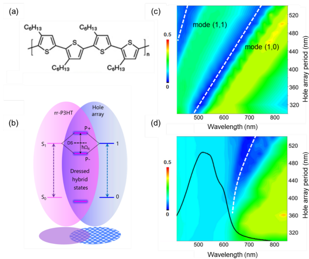
Figure 3.1. Strong coupling between surface plasmon and organic semiconductor: (a) Molecular structure of the p-type semiconductor rr-P3HT polymer. (b), Schematic representation of ultra-strong coupling between Ag hole array and rr-P3HT film. Contour image of transmission spectra of the hole arrays in the (c) absence and (d) presence of rr-P3HT (black curve shows the molecular absorption) as a function of period ranging from 320 nm to 540 nm
