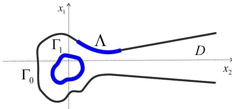
Figure 1 – Domain \Omega
