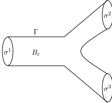
Figure 2 – Domain B_\epsilon
