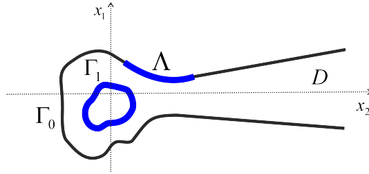
Figure 3.1 – Domain \Omega
