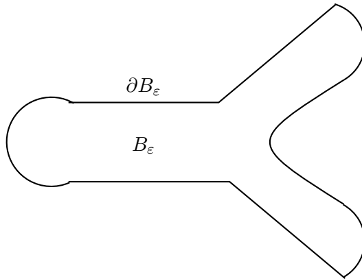
Figure 4 – Domain B_\varepsilon
