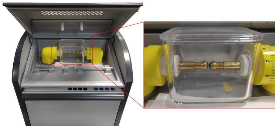
Figure 70 - Baur DPA-75C test showing the sphere-to-sphere electrode geometry and dielectric oil tank.
