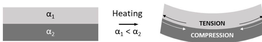
Figure 3 – Representation of reciprocal thermal stress experienced by bonded surfaces with mismatched CTE ( \alpha ) during a temperature increase. Left) Stress-free assembly at manufacturing temperature. Right) Stressed assembly during heating.
