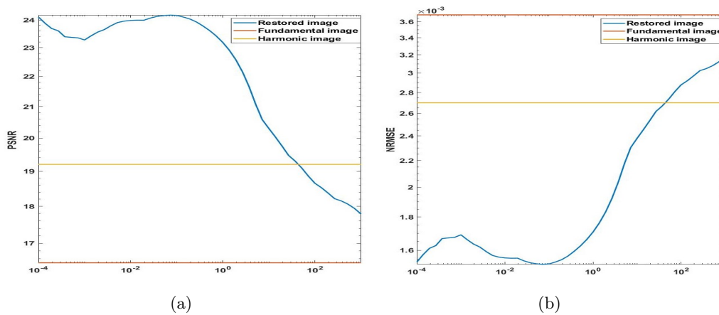
Figure 3.16: Illustration of the influence of the hyperparameter \beta on the result in terms of (a) PSNR and (b) NRMSE.
