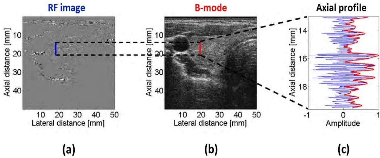
Figure 1.12: Relationship between RF and B-mode image for a thyroid image [Bas08]. (a) RF image, (b) B-Mode image, (c) an extraction of axial profile, RF signal in blue and corresponding envelope in red
