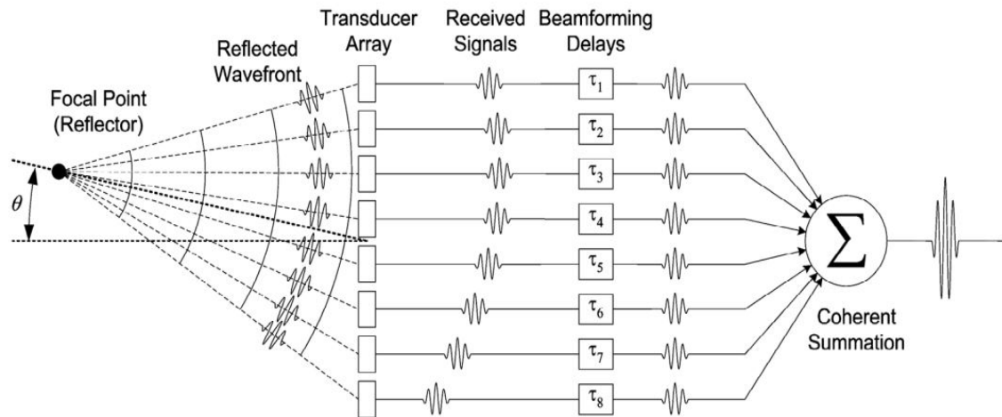
Figure 1.9: Delay-and-sum beamforming in a phased array ultrasound imaging system [JKKY05].
