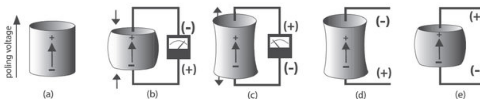
Figure 1.1: (a-c) Direct , (d-e) inverse piezoelectric effect [MF06].
