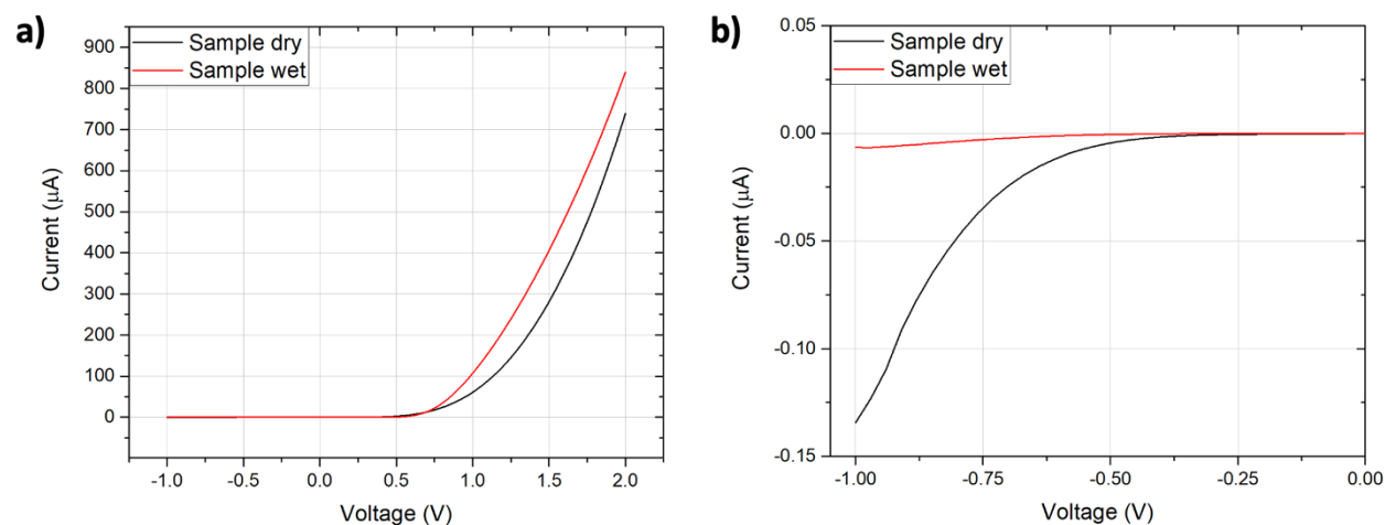
Figure 145: a) full I-V characteristics and b) reverse current comparison between cavities without holes in the base
