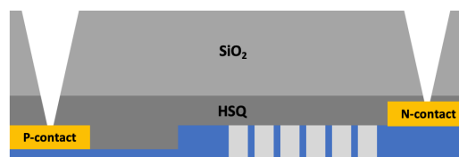
Figure 114: Schematics of the vias opening process
