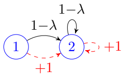
Figure 5.1.: Example in which the classical definition of indexability is ambiguous: All transitions are deterministic, and all labels on transitions indicate rewards. Solid black arrows correspond to the action “activate”, and dashed red arrows to the action “rest”.
