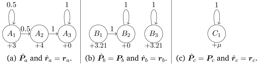
Figure 7.2.: Counterexample for OFU indices: \hat{\mathcal{B}}_a, \hat{\mathcal{B}}_b = \mathcal{B}_b, \hat{\mathcal{B}}_c = \mathcal{B}_c .
