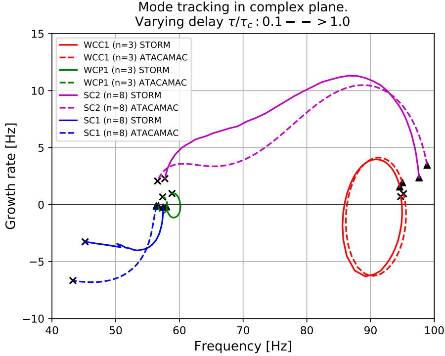
Figure 3.2: Trajectories of different modes in the complex-frequency plane for different flame interaction indices n and varying normalized flame-delay ( \tau/\tau_c ). ▲: Starting point, ×: last point of the trajectories. \tau_c is the time taken by an acoustic wave to traverse the chamber annulus.
