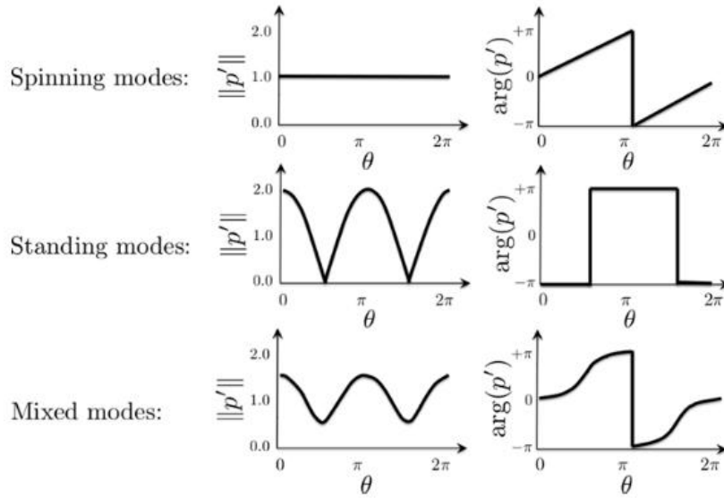
Figure 1.11: Structures of azimuthal acoustic eigenmodes: Spinning (top), standing (middle) and mixed (bottom) shown through the modulus and phase plots of complex acoustic pressure with respect to azimuthal coordinate \theta . Reproduced from [13].
