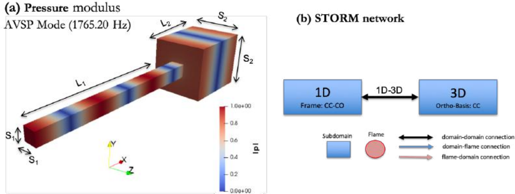
Figure 2.8: (a) System geometry. All global boundaries are presumed rigid walls. Dimensions and physical parameters in Tab. 2.2 below. Contours denote the magnitude |p| of complex-valued pressure Mode-4 (1765.20 Hz) from AVSP. (b) STORM network representation of this case.
