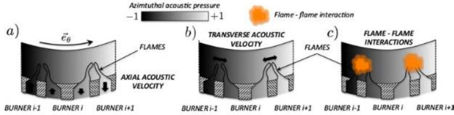
Figure 1.14: Flame dynamics mechanisms involved in azimuthal instabilities. Adapted from [111]
