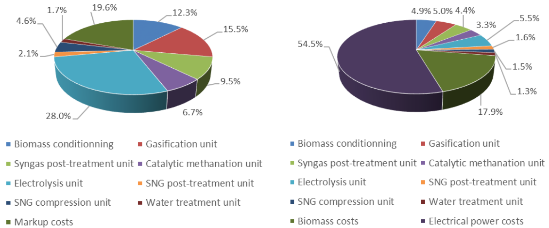
Figure 4-10: Total investment costs breakdown (left, total 21.9 €/MWh -1 ) and O&M costs breakdown (right, total 66.9 €/MWh -1 , total plant revenues excluded) in S2C
