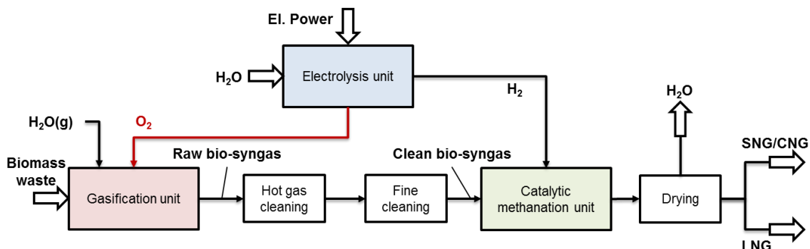
Figure 2-1: Schematic representation of investigated LNG or CNG plant concepts for bio-syngas upgrading [9]
